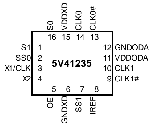
16-pin QFN
