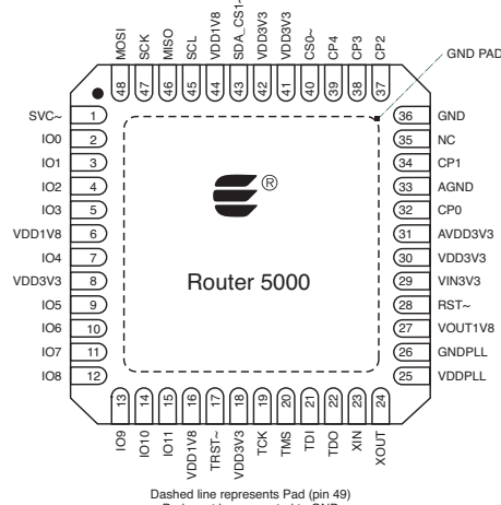
Figure 2: Router 5000 Pinout
