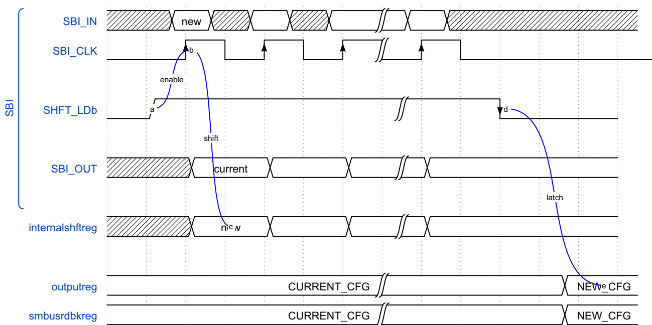
Figure 33. Side-Band Interface Functional Timing
