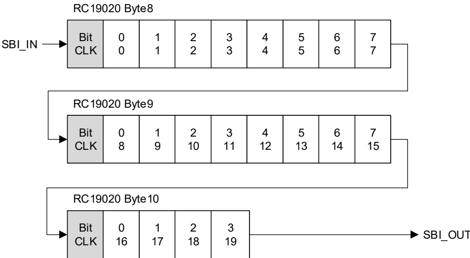
Figure 28. RC19020A Side-Band Shift Order
