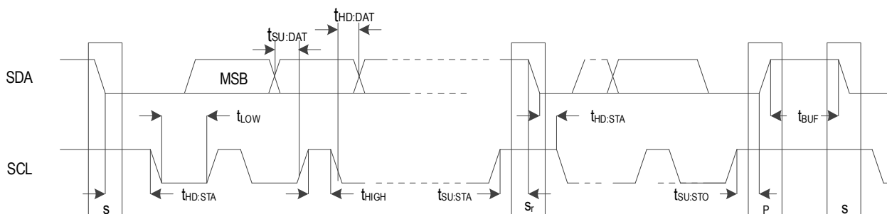
Figure 10. SMBus Slave Timing Diagram
