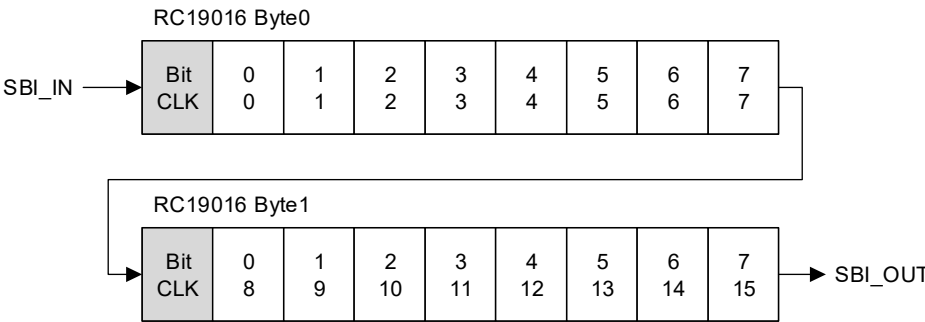
Figure 29. RC19016A Side-Band Shift Order
