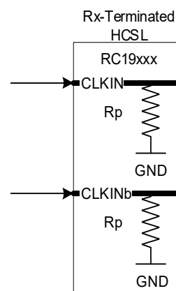
Figure 18. Receiver Termination
