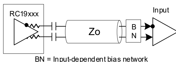
Figure 21. AC-Coupled
