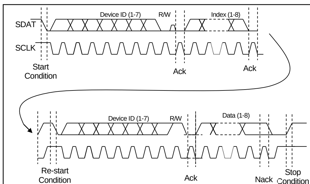
FIGURE 28. ONE COMPLETE REGISTER READ SEQUENCE VIA THE SERIAL BUS INTERFACE
