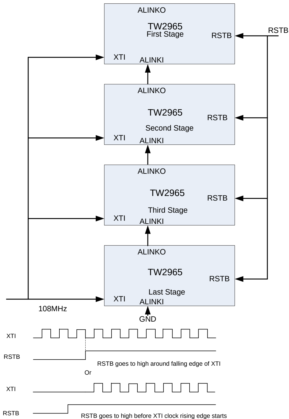
FIGURE 12. RSTB CONTROL FOR 108MHZ XT INPUT
