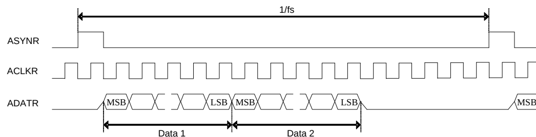
FIGURE 16. ACLMASTER=0, RM_SYNC=1
