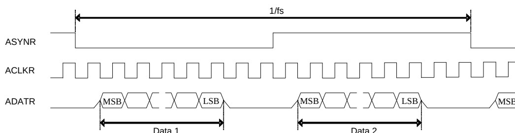
FIGURE 15. ACLMASTER=0, RM_SYNC=0
