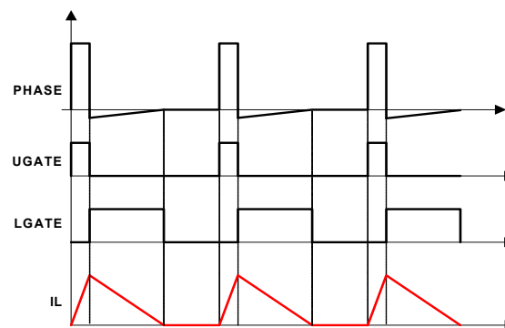
FIGURE 28. DIODE EMULATION
