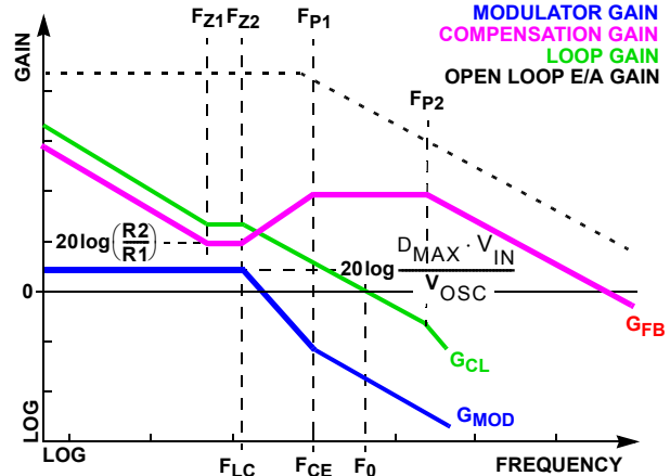
FIGURE 16. ASYMPTOTIC BODE PLOT OF CONVERTER GAIN
