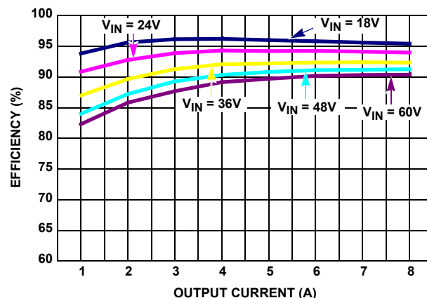
FIGURE 8. EFFICIENCY VS LOAD (OUTPUT VOLTAGE = 12V, F_{SW} = 200\text{kHz} (SEE APPLICATION NOTE FOR MORE DETAILS))
