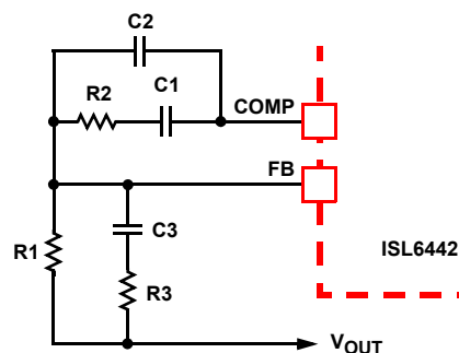
FIGURE 13. COMPENSATION CONFIGURATION FOR ISL6442 CIRCUIT
