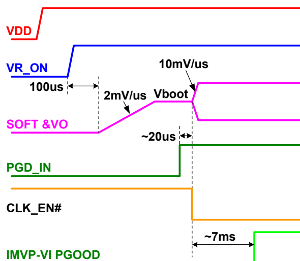
FIGURE 4. SOFT-START WAVEFORMS USING A 20nF SOFT CAPACITOR
