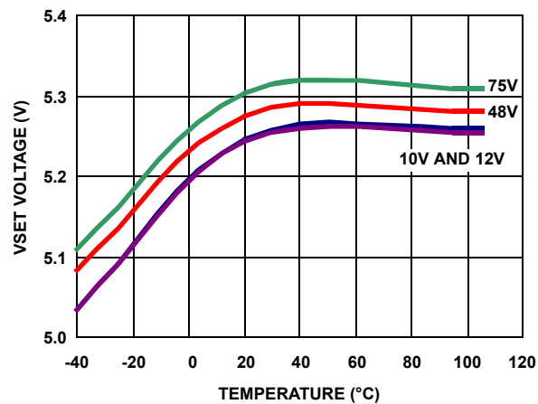
FIGURE 7. VSET VOLTAGE
