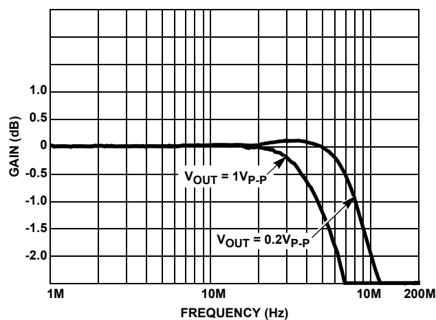
FIGURE 13. GAIN FLATNESS
