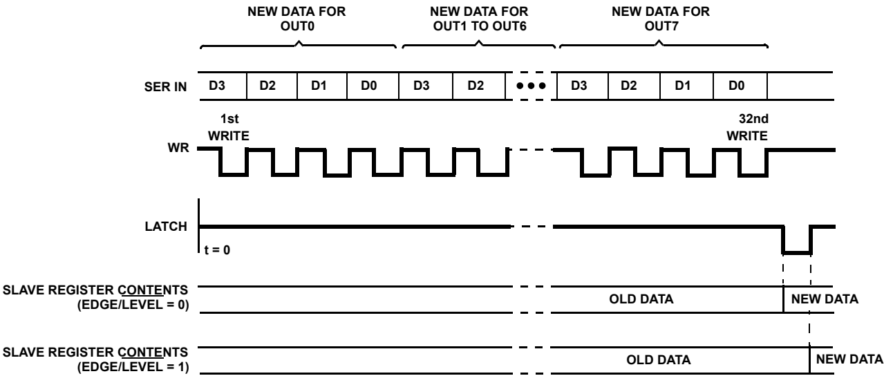
FIGURE 5. SERIAL PROGRAMMING MODE OPERATION ( \overline{\text{SER/PAR}} = 1 )
