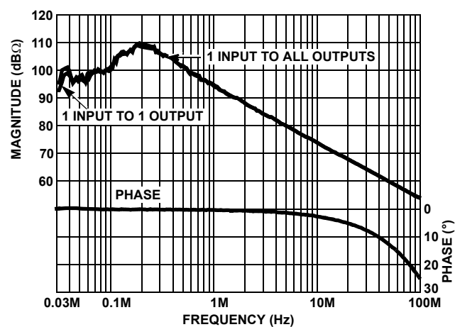
FIGURE 17. INPUT IMPEDANCE vs FREQUENCY
