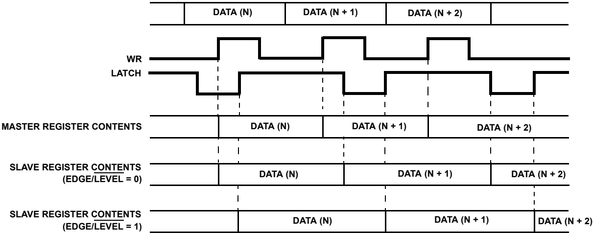
FIGURE 4. PARALLEL PROGRAMMING MODE OPERATION ( \overline{\text{SER/PAR}} = 0 )
