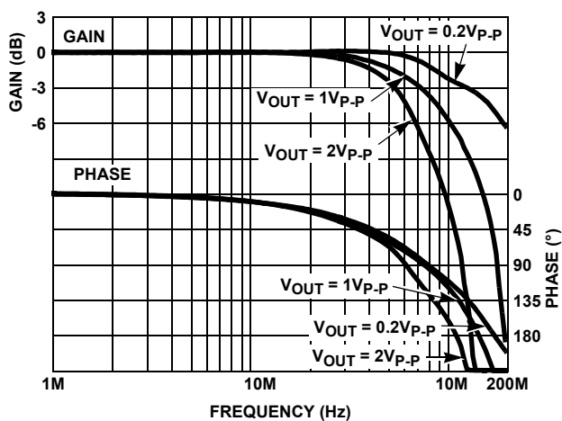
FIGURE 12. FREQUENCY RESPONSE
