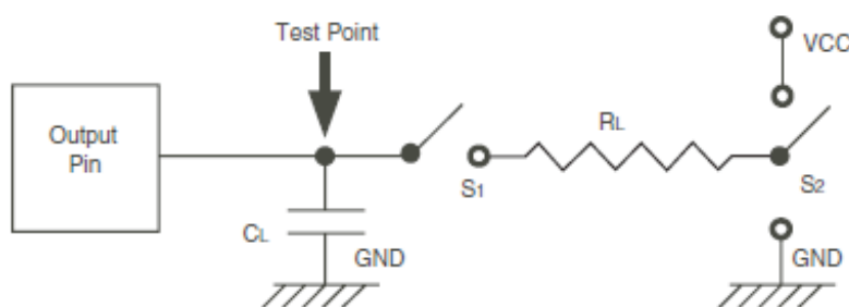
Figure 6. Output Load
