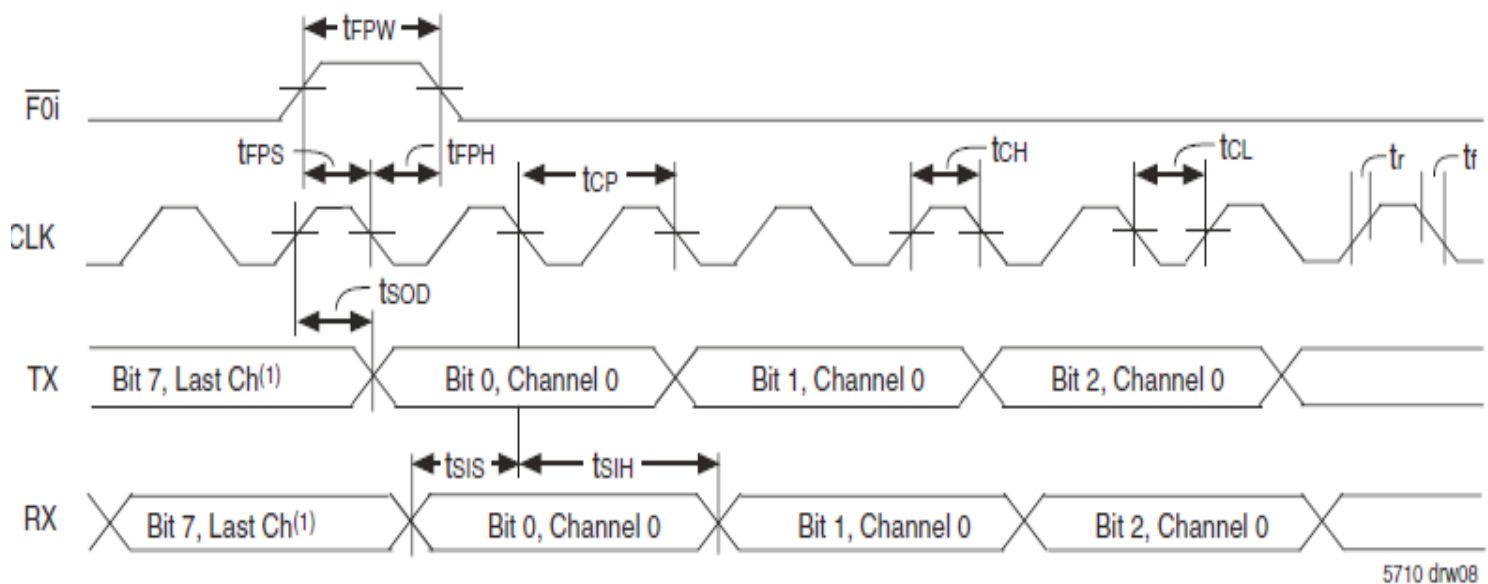
Figure 8. GCI Timing when WFPS pin = 0
