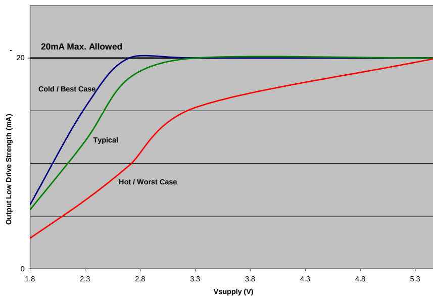
Figure 7.2 Output Low Drive Strength Graph
