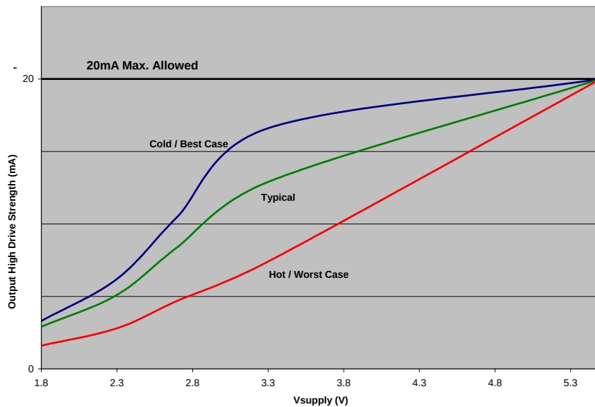
Figure 7.1 Output High Drive Strength Graph
