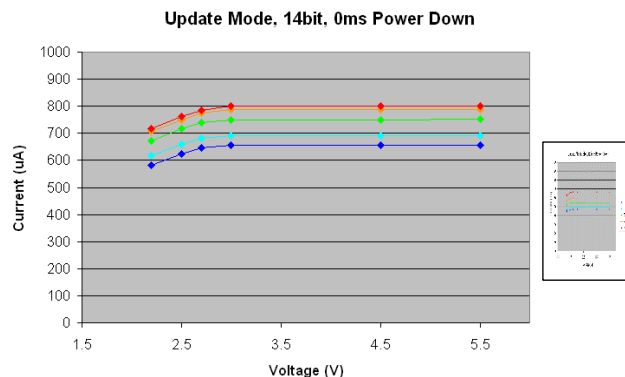
Figure 6.2 Worst Case Settings (Typical Part)
