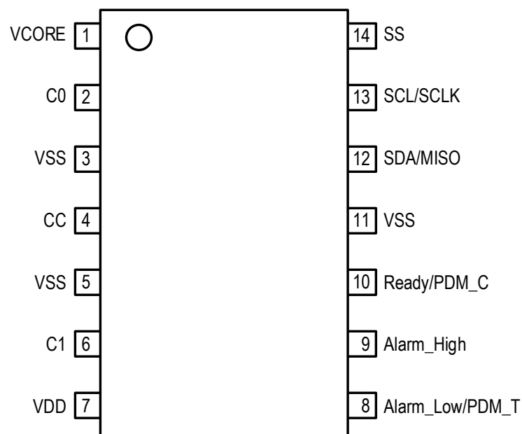
Figure 1.1 Pin Assignments for 4.4 \times 5.0 mm 14-TSSOP – Top View
