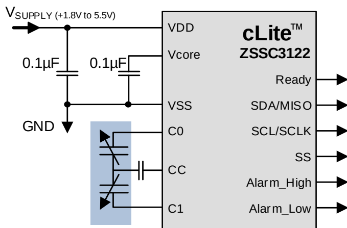
Figure 14.4 Differential Input Capacitance Example
