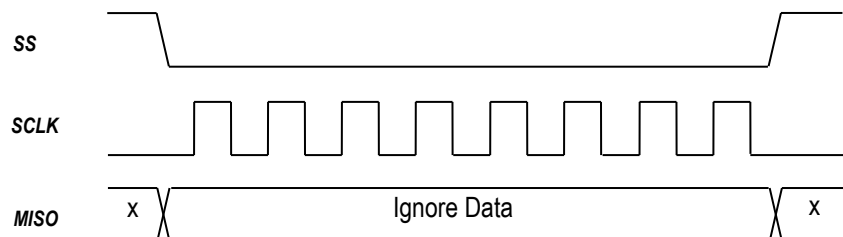
Figure 10.13 SPI MR
