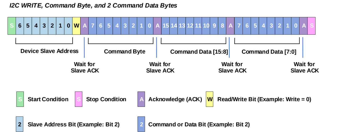
Figure 11.1 I2C Command Format
