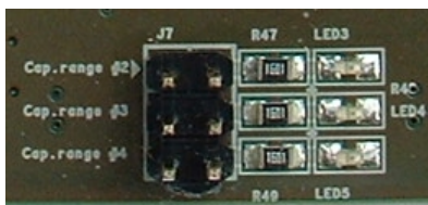
Figure 4.1 J7 – Output Capacitor Range Hardware Selection
