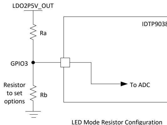
Figure 3. P9038 LED Resistor Optioning
