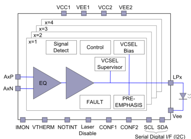
Figure 1: Device diagram
