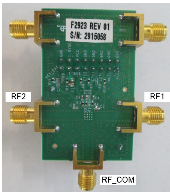
Bottom View
