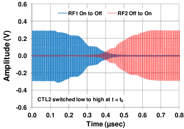
Switching Time T_c=-40^\circ\text{C} [RF_COM Driven, RF1 to RF2]
