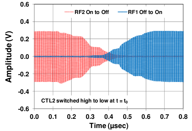
Switching Time T_c=-40^\circ\text{C} [RF_COM Driven, RF2 to RF1]
