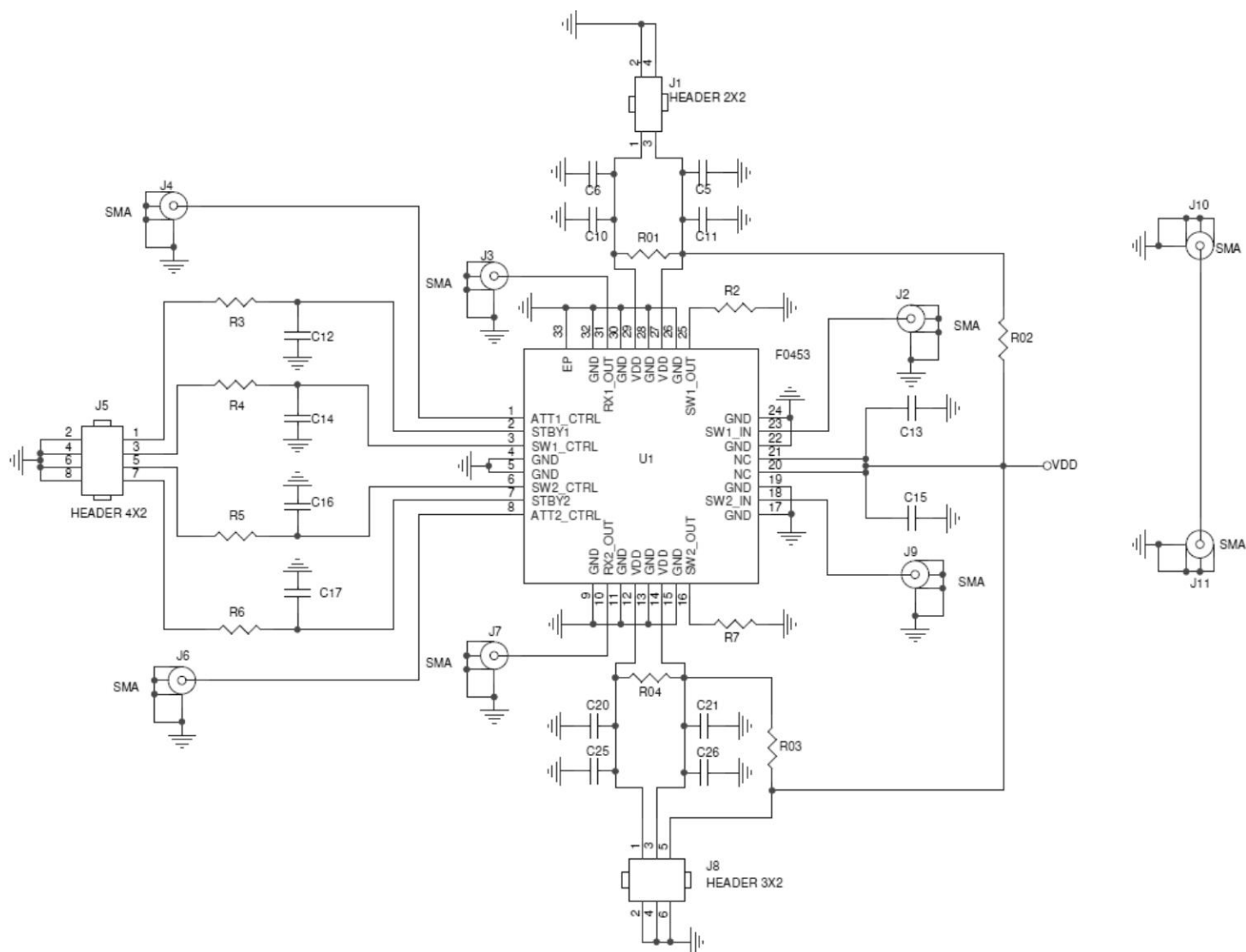
Figure 29. Electrical Schematic
