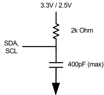
Figure 6: AC Output Test Load (I²C)
