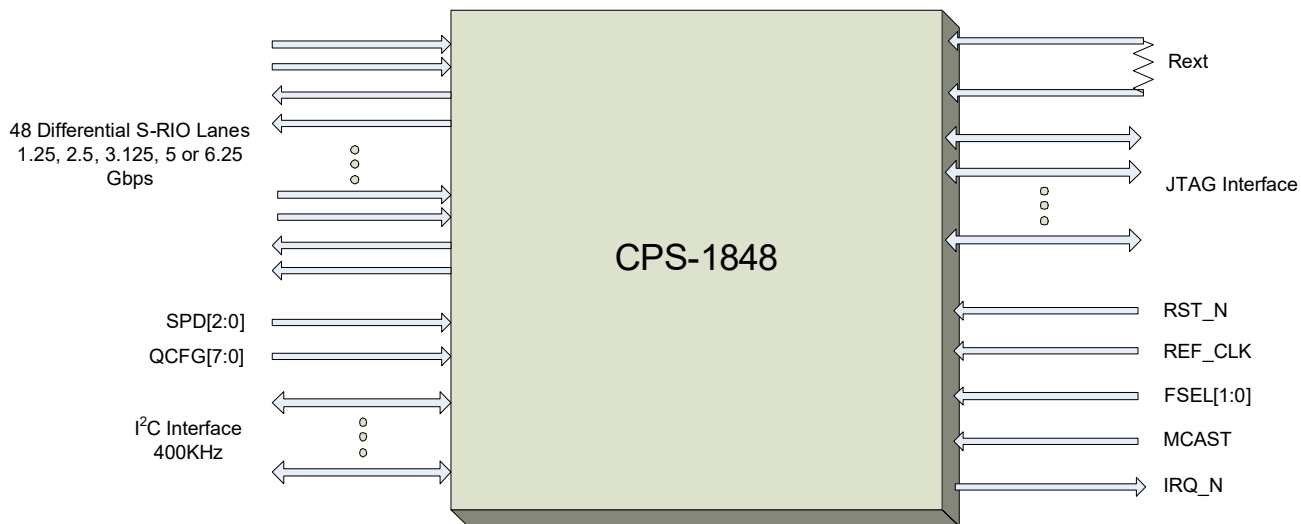
Figure 1: CPS-1848 Interfaces
