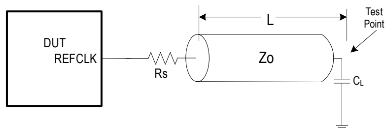
Figure 4. Single-ended Output Test Load
