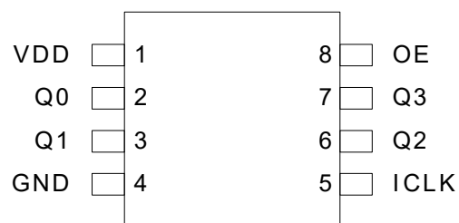
8-pin SOIC
