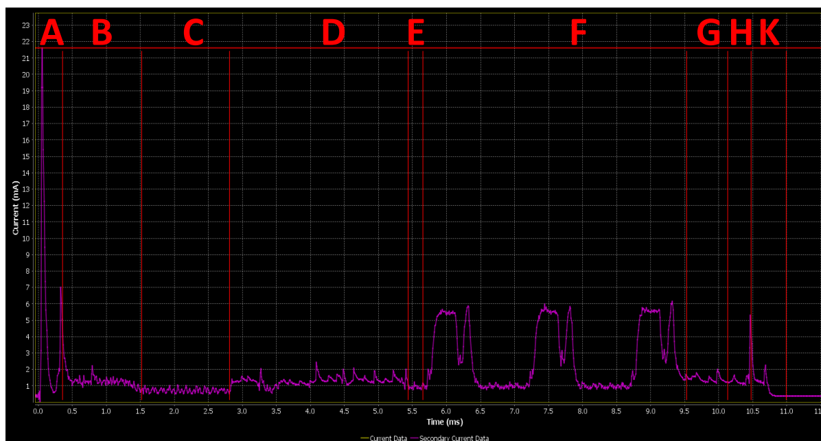
Figure 122: BLE Advertising power profile
