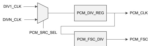
Figure 61: PCM clock generation
