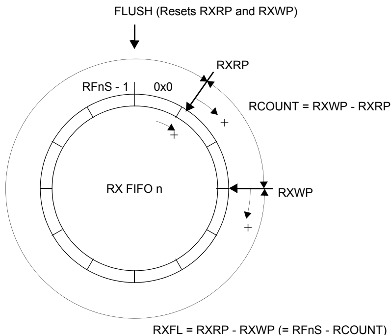
Figure 110: Rx FIFO operation
