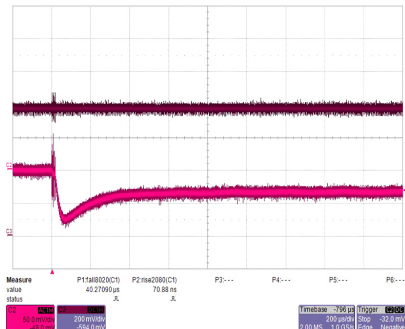
Figure 16: LDO_VBAT_RET loadstep 0 to 5mA (Cload=4.7 \mu F, Vout=2.4V)
