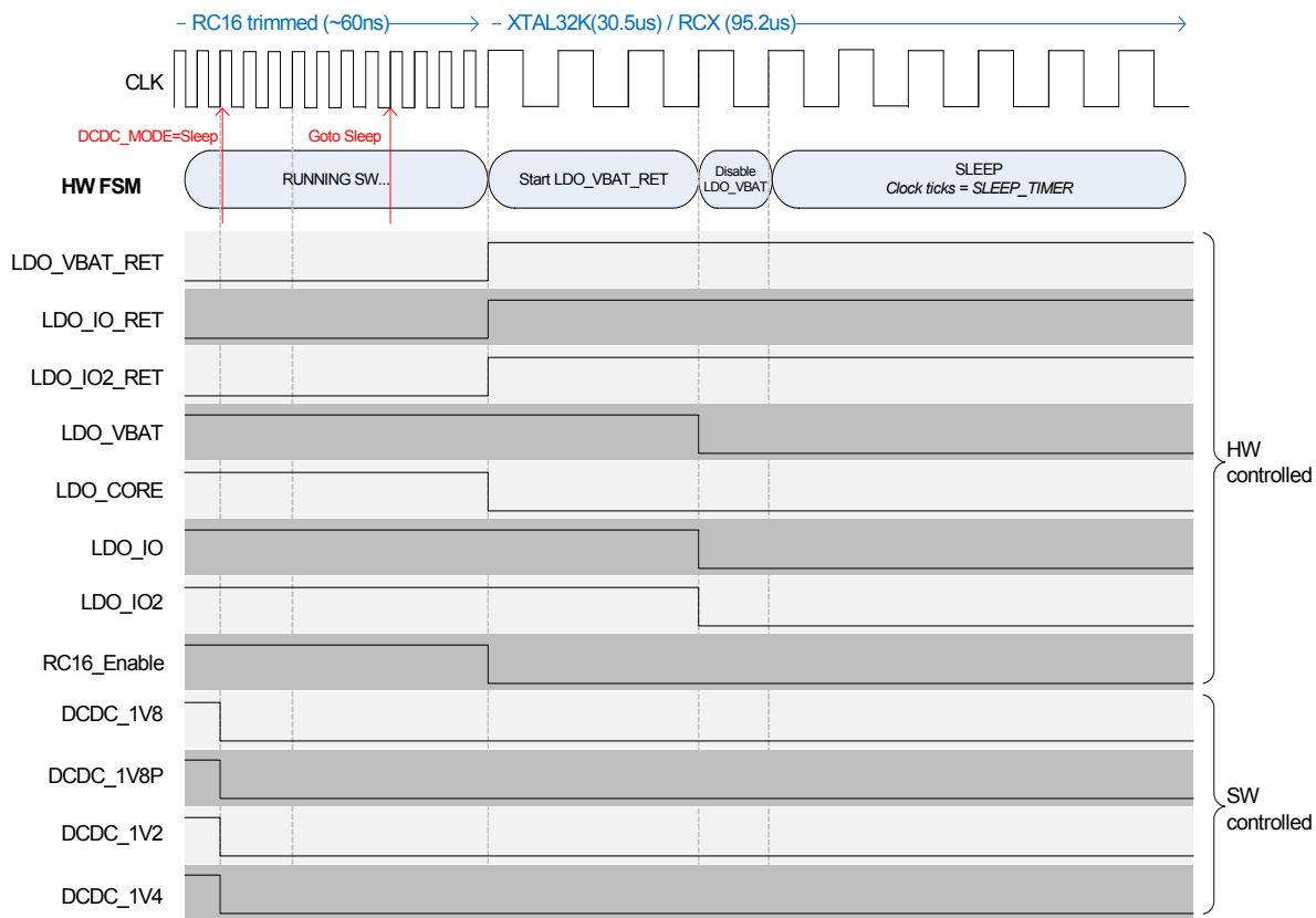
Figure 18: Goto Sleep timing and PMU operations
