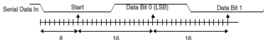
Figure 69: Receiver Serial Data Sample Points
