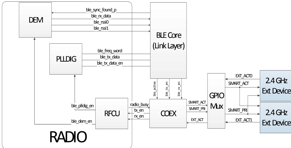
Figure 124: Coexistence interface
