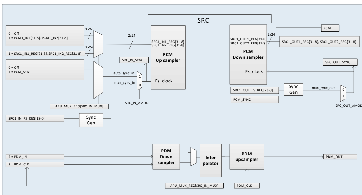
Figure 56: Sample rate Converter block diagram
