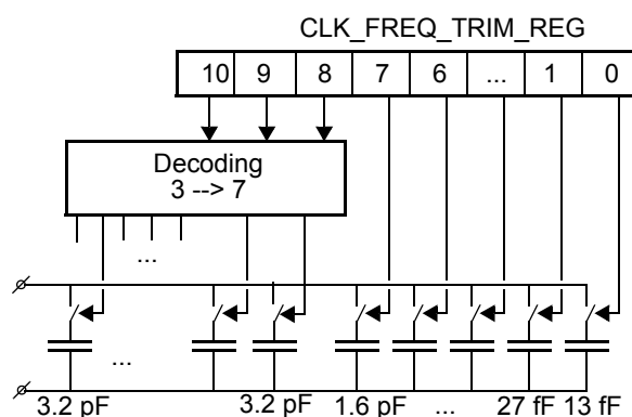
Figure 29: Frequency trimming
