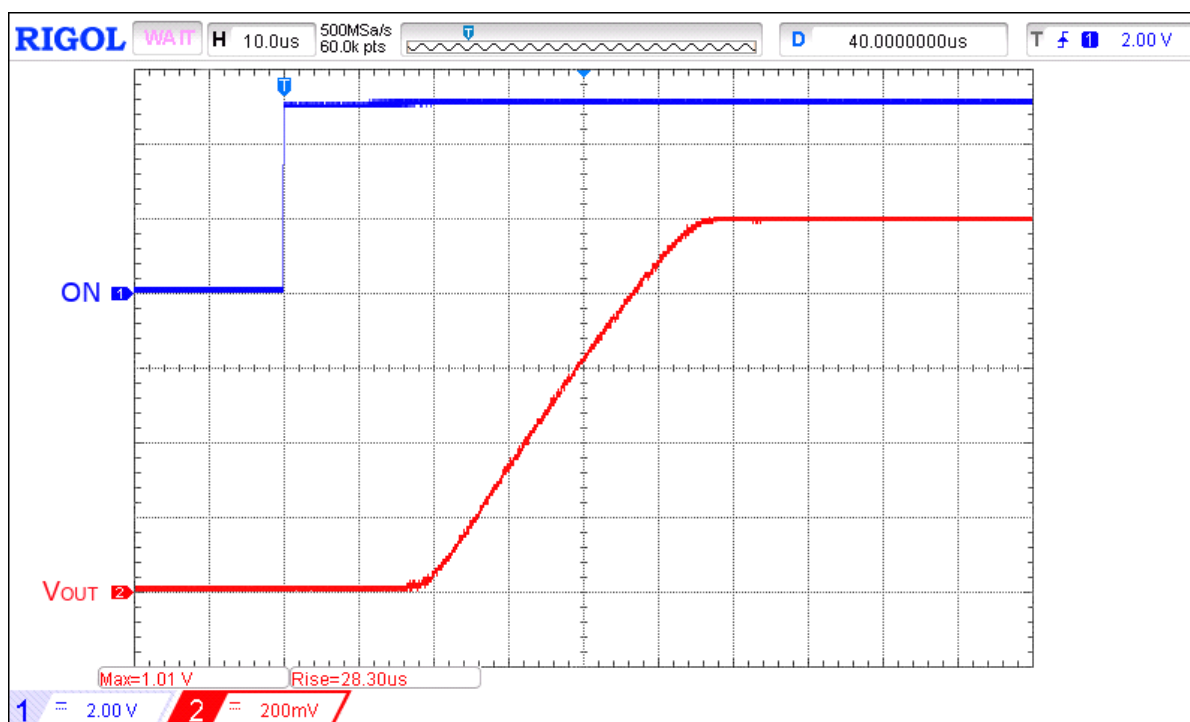
Figure 1. Typical Turn ON operation waveform for V_{DD} = 5\text{ V} , V_{IN} = 1\text{ V} , C_{SLEW} = 4.7\text{ nF} , C_{LOAD} = 10\text{ μF} , R_{LOAD} = 20\text{ Ω}
