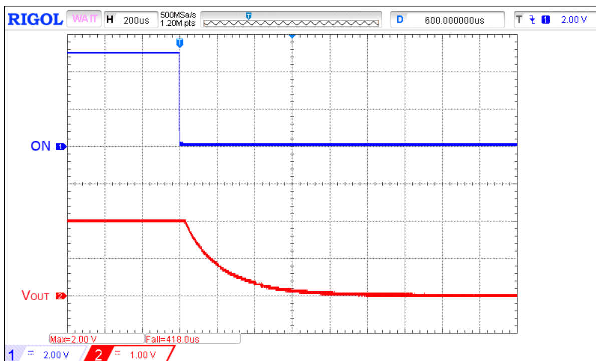
Figure 11. Typical Turn OFF operation waveform for V_{DD} = 5\text{ V} , V_{IN} = 1.98\text{ V} , C_{SLEW} = 4.7\text{ nF} , C_{LOAD} = 10\text{ μF} , R_{LOAD} = 20\text{ Ω}
