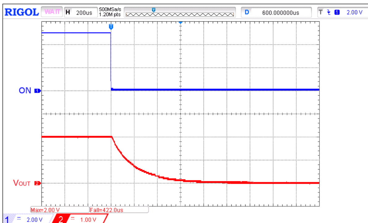
Figure 12. Typical Turn OFF operation waveform for V_{DD} = 5\text{ V} , V_{IN} = 1.98\text{ V} , C_{SLEW} = 22\text{ nF} , C_{LOAD} = 10\text{ μF} , R_{LOAD} = 20\text{ Ω}
