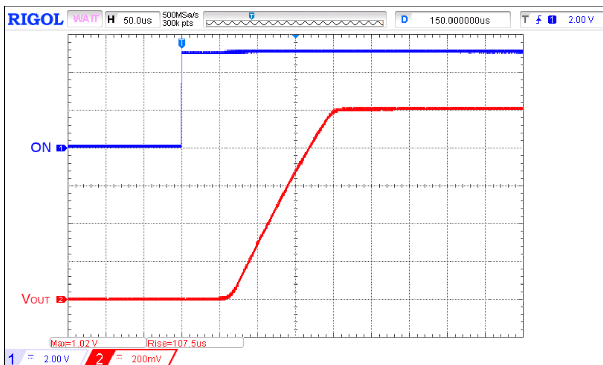
Figure 2. Typical Turn ON operation waveform for V_{DD} = 5\text{ V} , V_{IN} = 1\text{ V} , C_{SLEW} = 22\text{ nF} , C_{LOAD} = 10\text{ μF} , R_{LOAD} = 20\text{ Ω}
