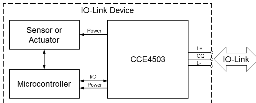
Figure 1: System Diagram
