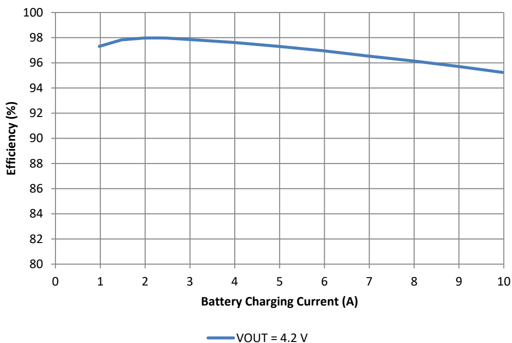
Figure 7: DA9318M Efficiency
