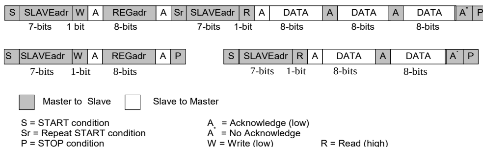
Figure 18: Page Read
