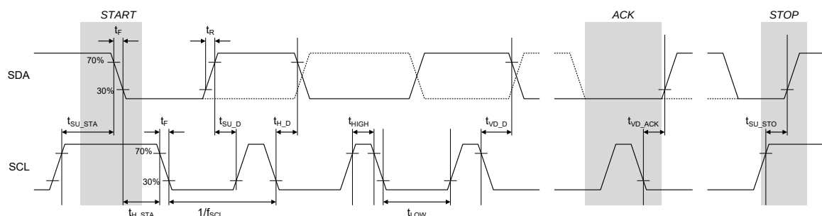
Figure 3: Interface Timing
