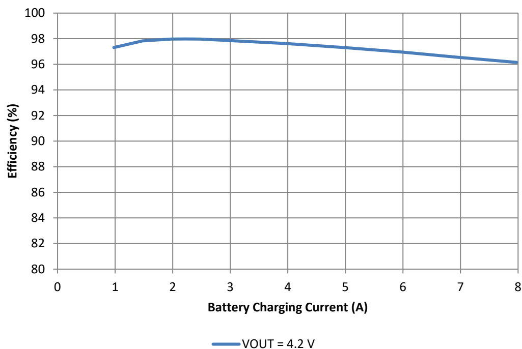
Figure 4: DA9318L Efficiency
