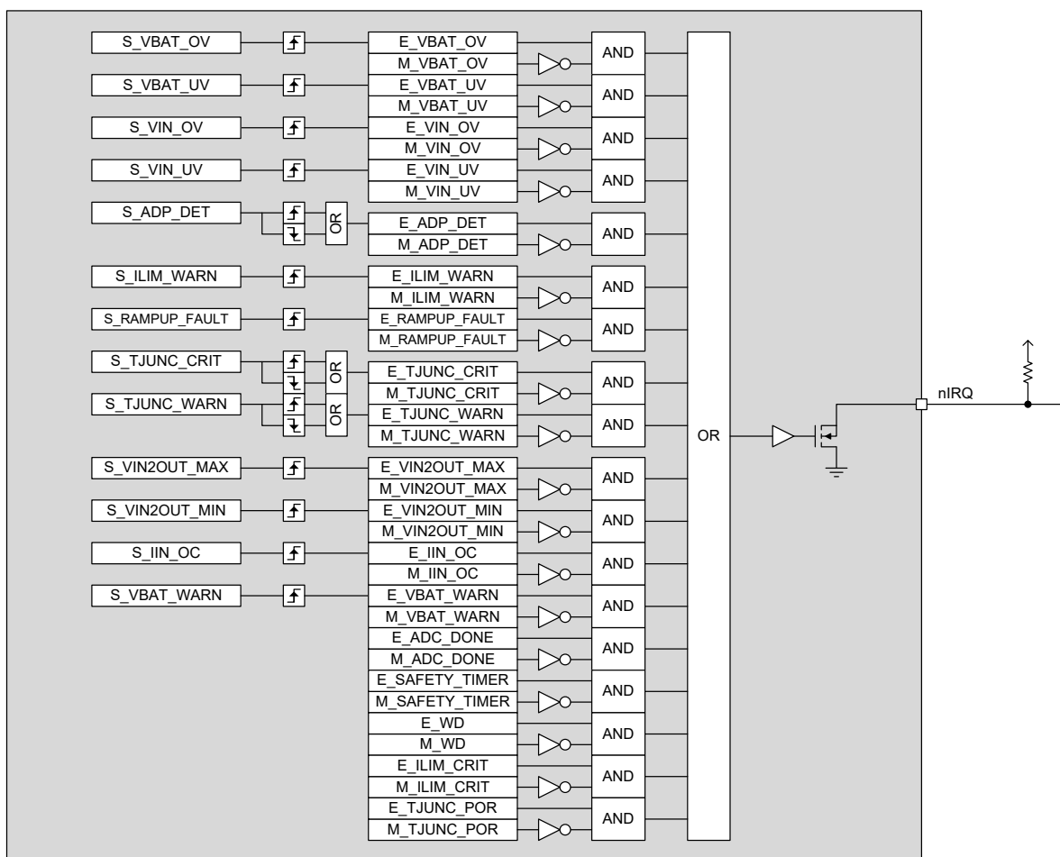
Figure 14: Interrupt Logic
