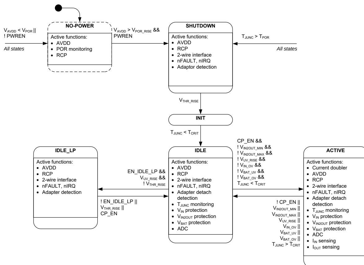
Figure 22: Power Modes
