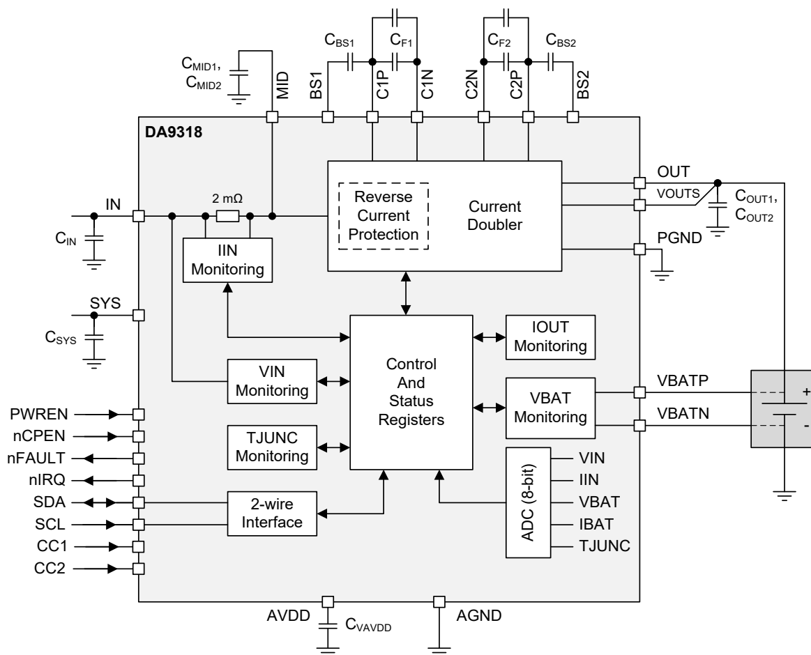
Figure 1: Block Diagram
