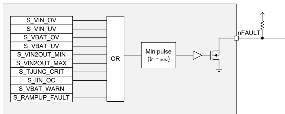
Figure 13: nFAULT Operation
