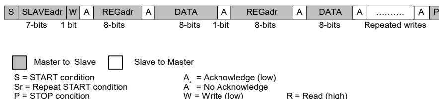
Figure 20: Repeated Write
