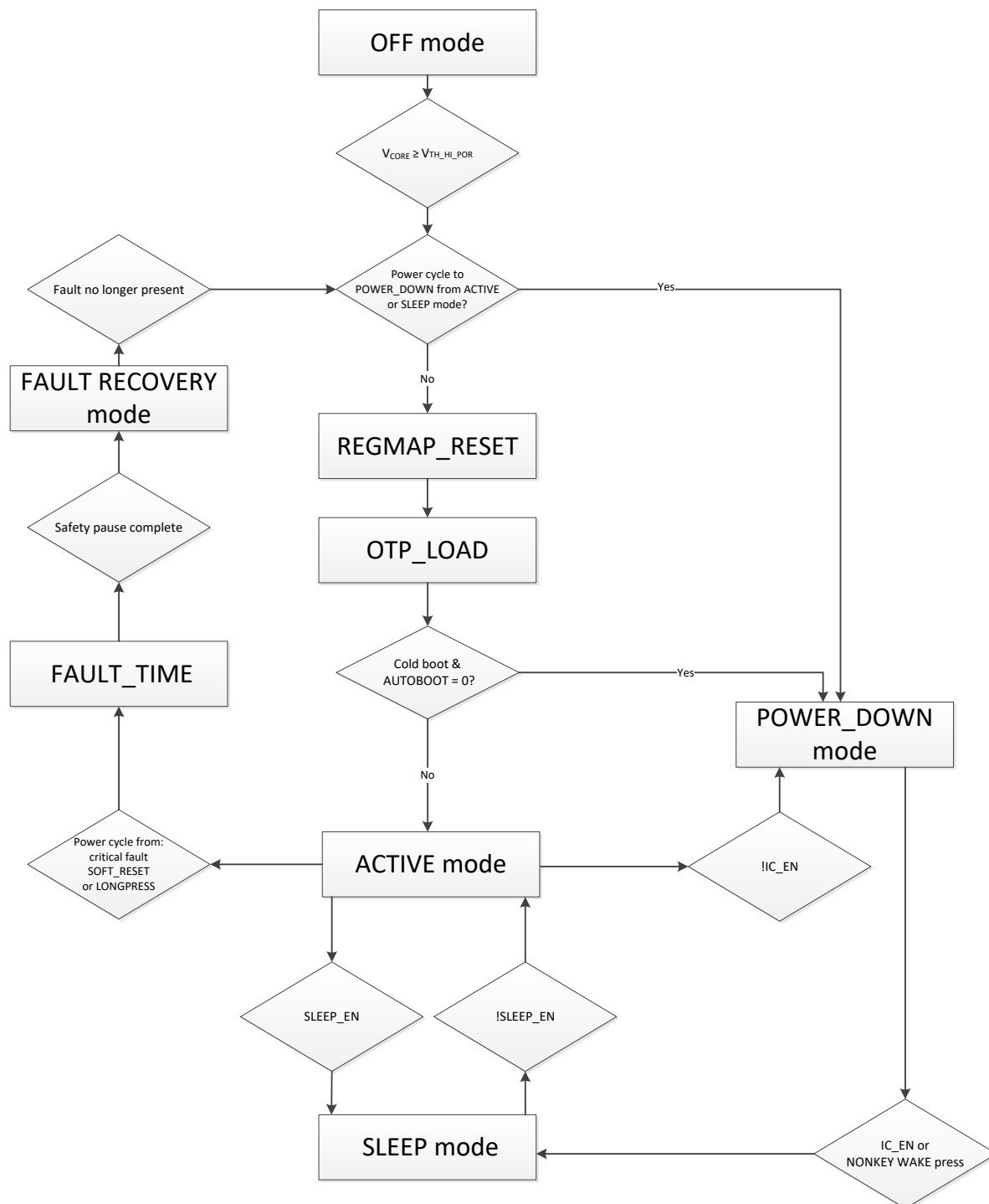
Figure 14: Operating Modes
