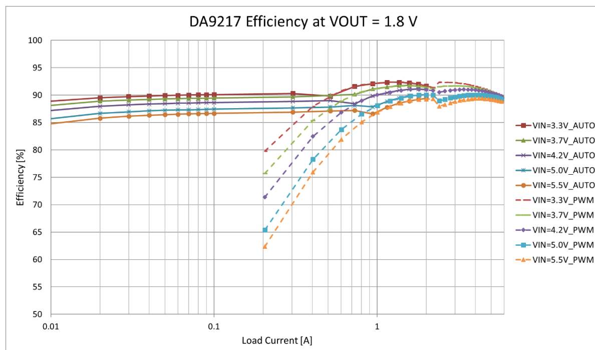
Figure 9: Efficiency vs Load, V_{OUT} = 1.8\text{ V}
