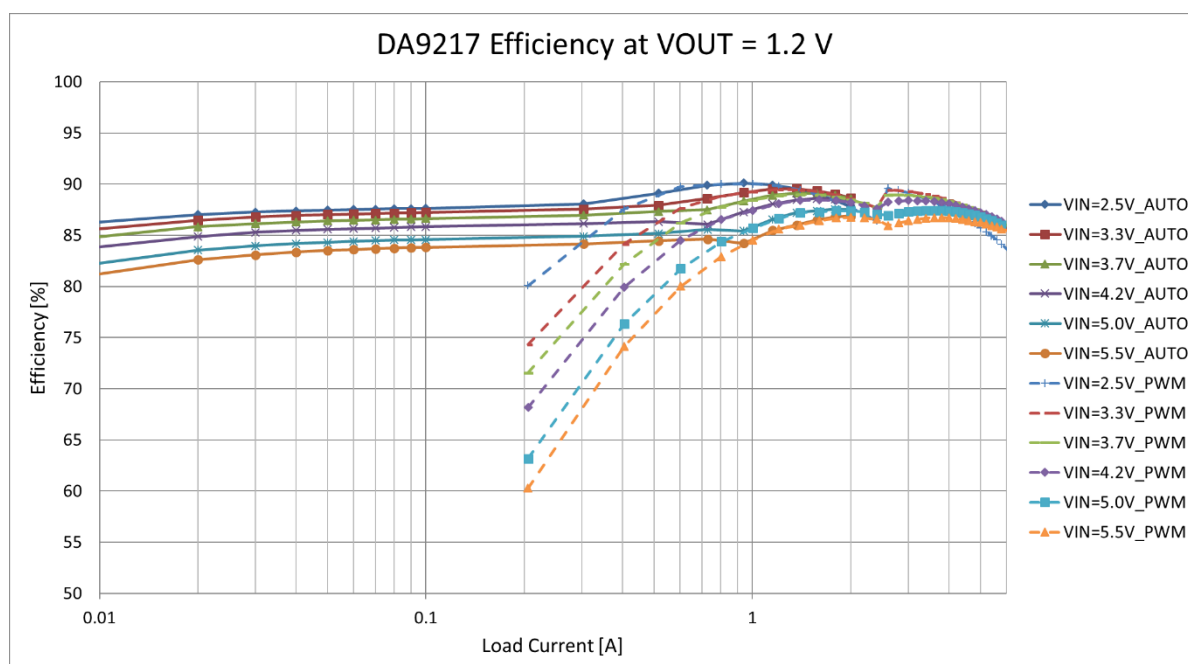
Figure 8: Efficiency vs Load, V_{OUT} = 1.2\text{ V}
