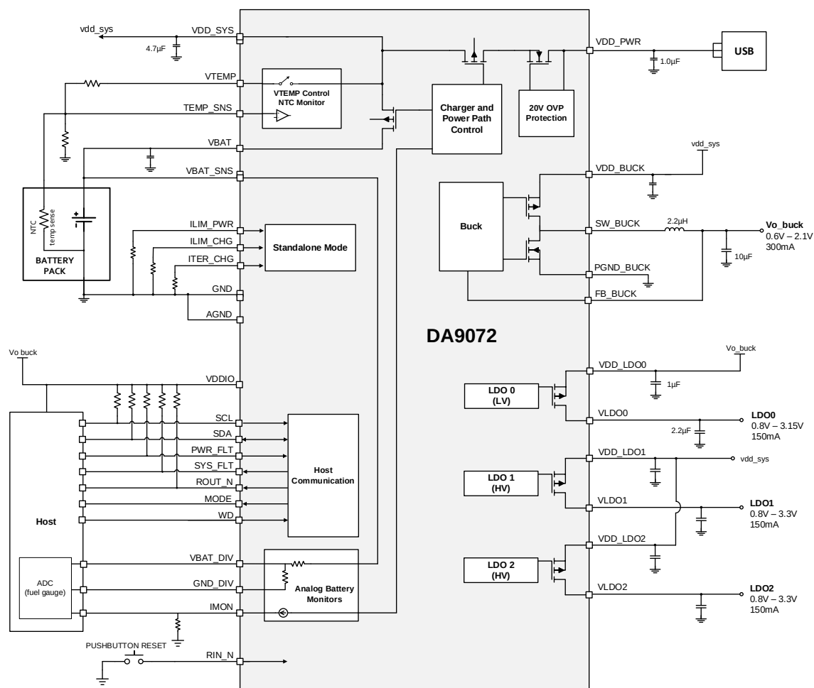
Figure 1: System Diagram
