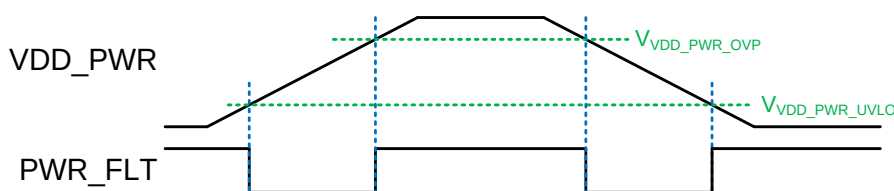
Figure 30: PWR_FLT Configured as VDD_PWR Status Indicator
