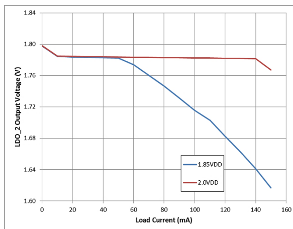
Figure 14: LDO2 Regulation and Dropout, V_{OUT} = 1.80\text{ V}
