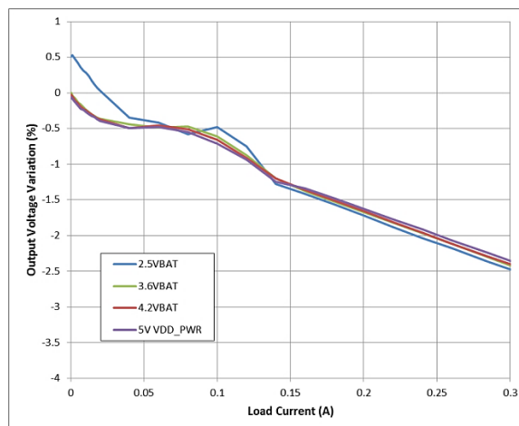
Figure 4: Buck Regulation, V_{OUT} = 1.8\text{ V}
