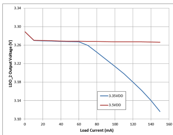
Figure 12: LDO2 Load Regulation, V_{OUT} = 3.30\text{ V}
