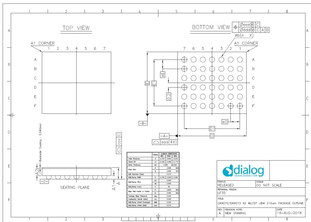
Figure 36: WLCSP-42 Package Outline Drawing, OH version
