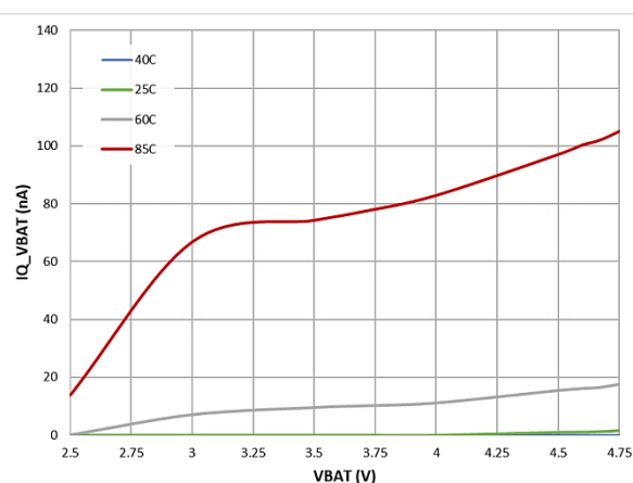
Figure 16: VBAT I_Q , Ship Mode
