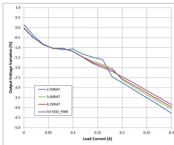
Figure 6: Buck Regulation, V_{OUT} = 0.9\text{ V}
