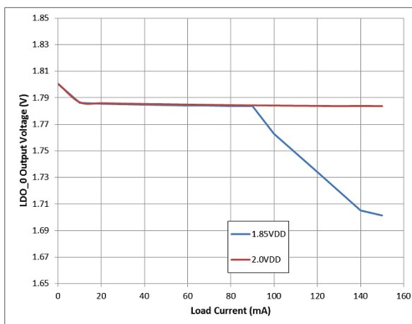
Figure 8: LDO0 Regulation and Dropout, V_{OUT} = 1.80\text{ V}
