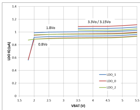
Figure 18: VDD_LDO I_Q , No Load
