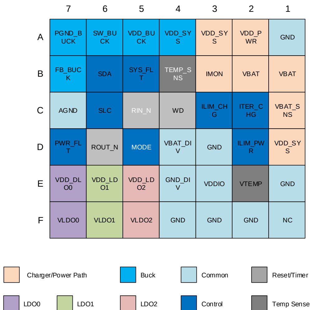
Figure 2: Pinout Diagram (Bottom View)
