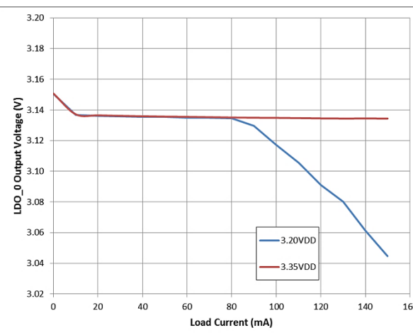
Figure 10: LDO0 Regulation and Dropout, V_{OUT} = 3.15\text{ V}
