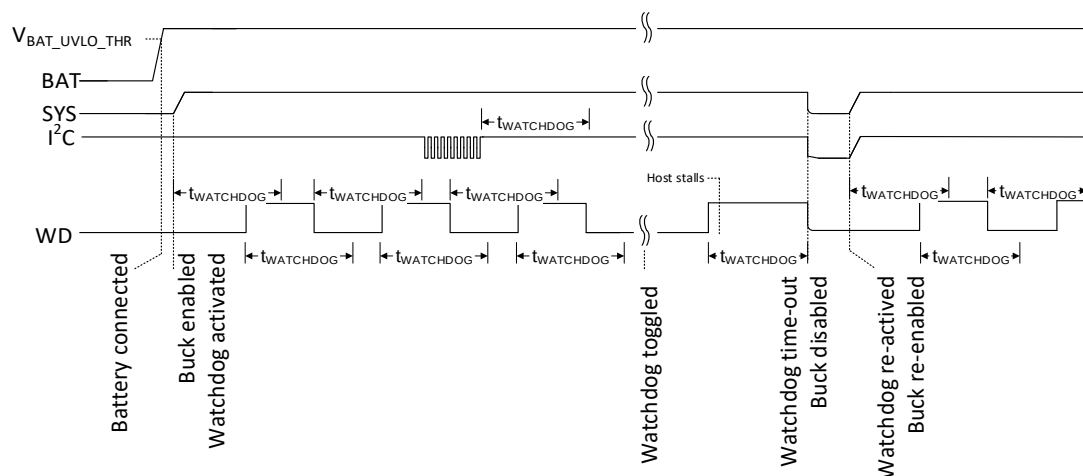
Figure 28: Watchdog Behavior
