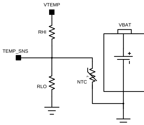
Figure 29: Battery Temperature Sensing with NTC
