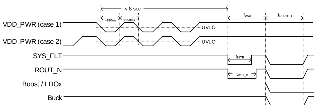
Figure 34: Power-Cycle by VDD_PWR Insertion
