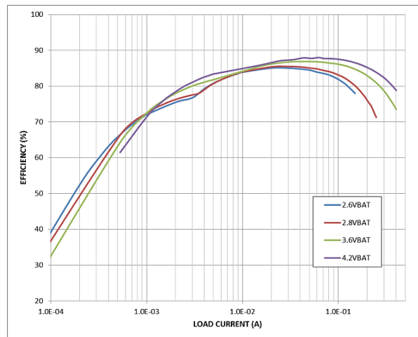
Figure 10: Boost Efficiency, V_{OUT} = 5\text{ V} , V_{IN} = V_{BAT}
