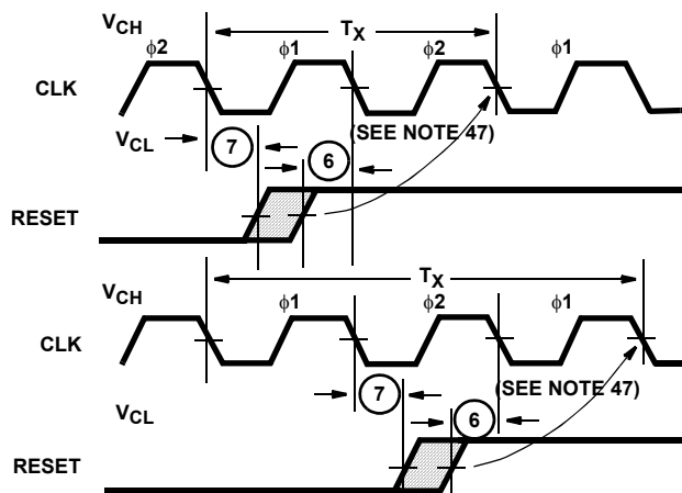
FIGURE 36. 80C286 RESET INPUT TIMING AND SUBSEQUENT PROCESSOR CYCLE PHASE
