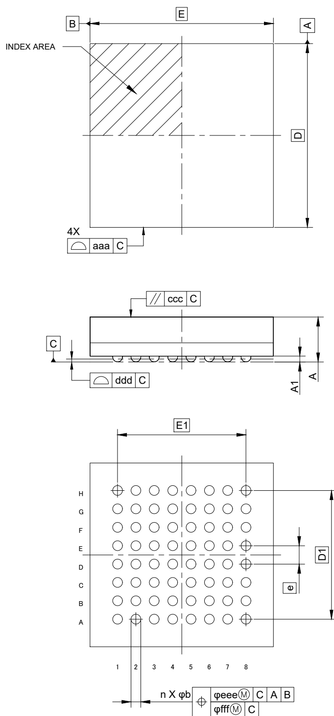
Figure 2.4 BGA 64-pin
