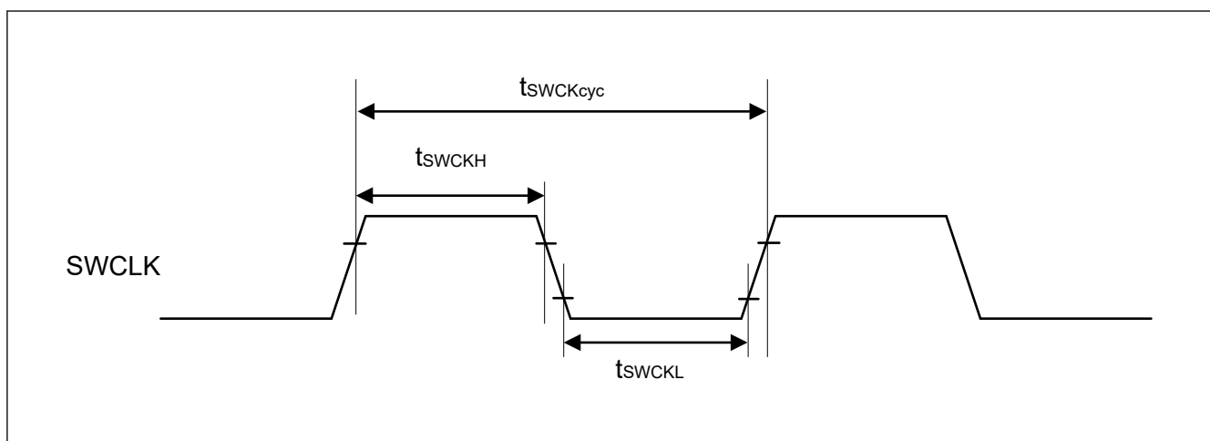
Figure 2.62 SWD SWCLK timing
