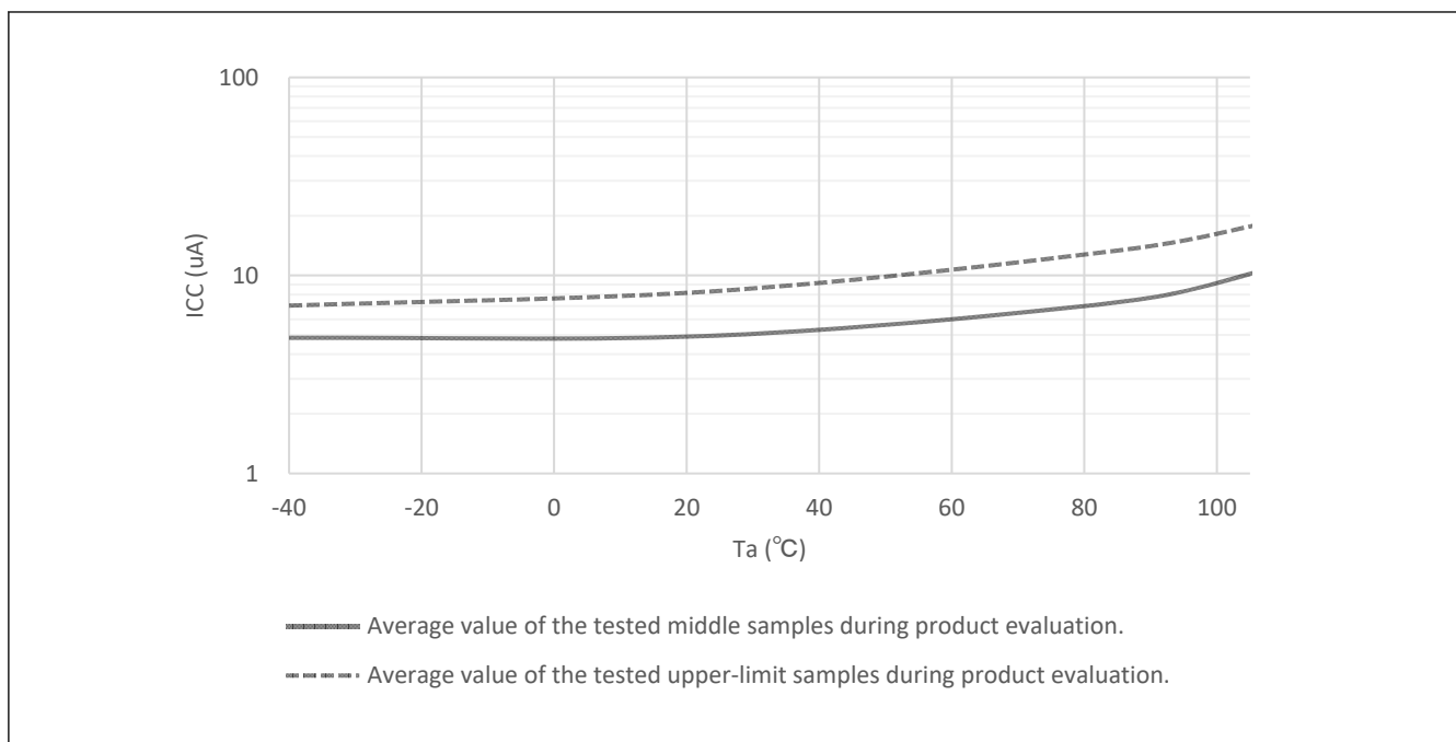
Figure 2.5 Temperature dependency in Deep Software Standby mode, DPSBYCR.DEEPCUT[1:0] = 11b (reference data)
