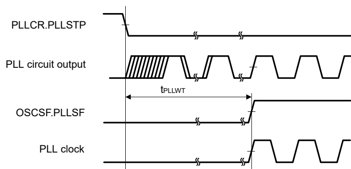
Figure 2.10 PLL clock oscillation start timing
