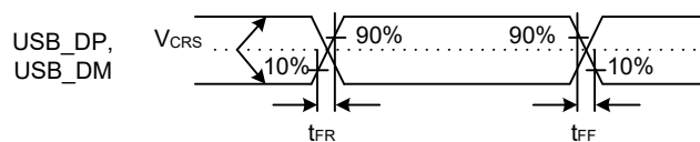
Figure 2.53 USB_DP and USB_DM output timing in full-speed mode
