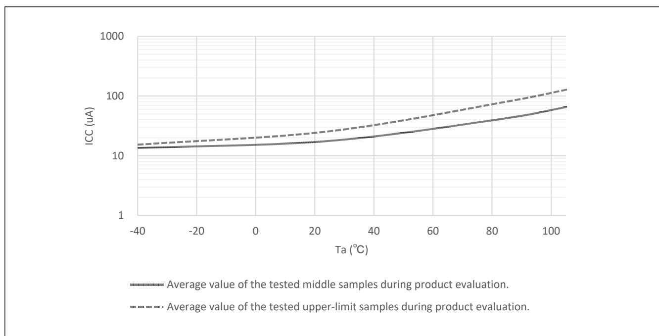
Figure 2.3 Temperature dependency in Deep Software Standby mode, \text{DPSBYCR.DEEPCUT}[1:0] = 00\text{b} (reference data)
