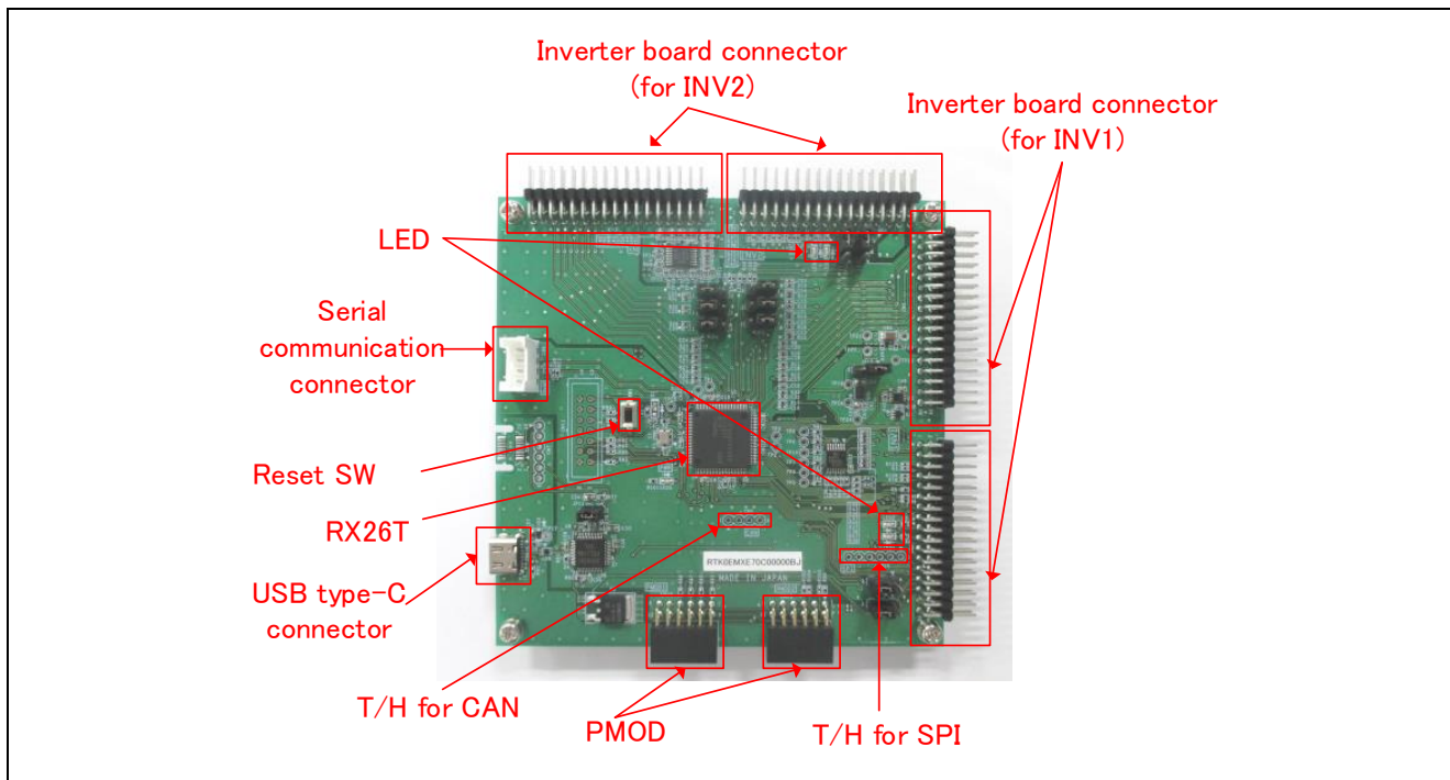
Figure 4-2 CPU Board Layout
