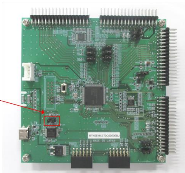
Figure 5-1 JP11 setting
