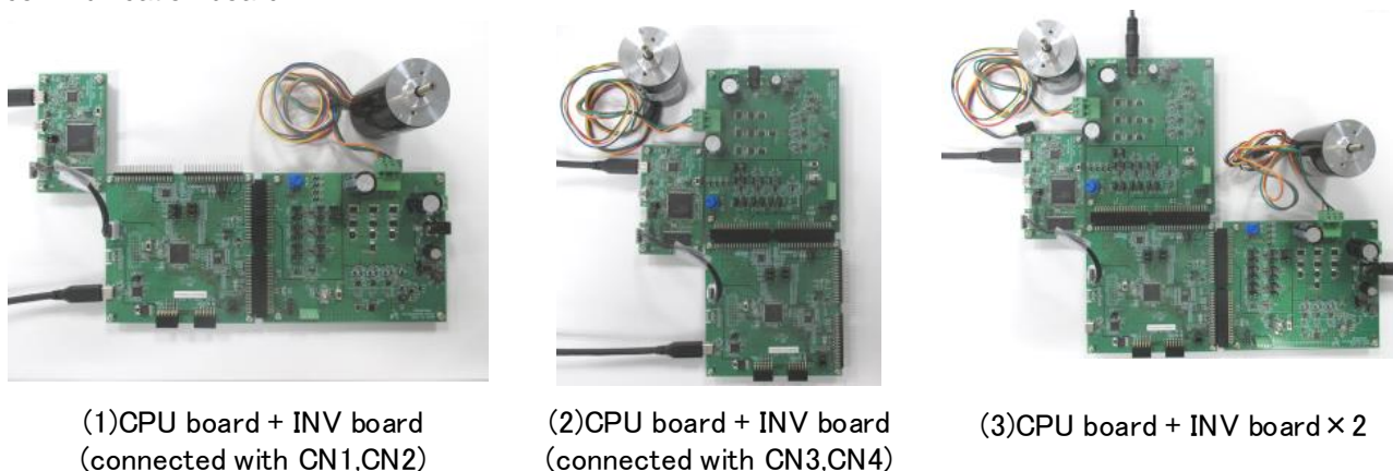
Figure 5-1 Board connection of CPU board, INV board and COM board
