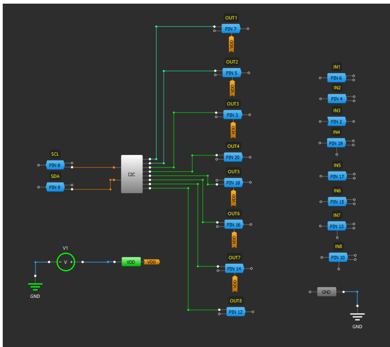
Figure 3-11 SLG46537V (IC13) input and output internal configuration.
