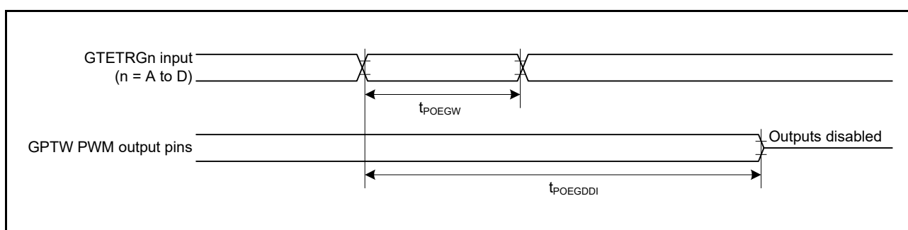
Figure 2.30 Output Disable Time for POEG in Direct Response to the Input Level Detection of the GTETRn pin
