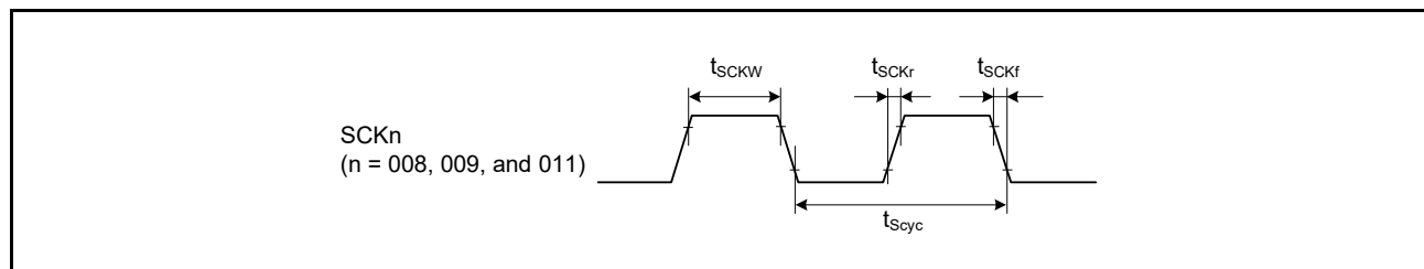
Figure 2.44 SCK Clock Input Timing
