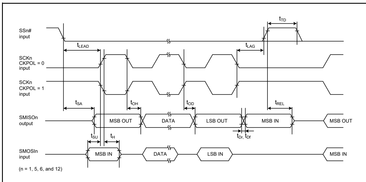
Figure 2.42 Simple SPI Timing (Slave, CKPH = 1)
