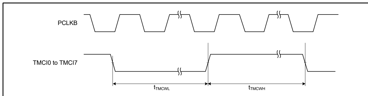
Figure 2.15 TMR Clock Input Timing
