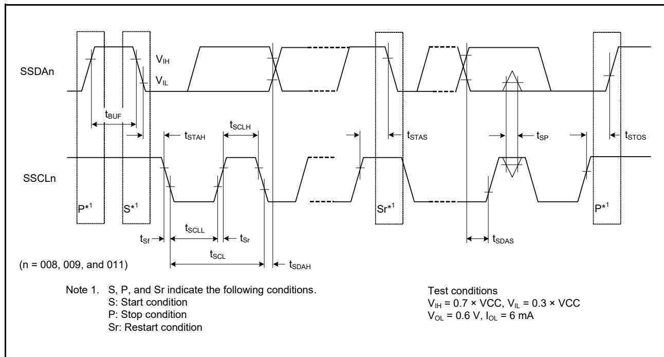
Figure 2.46 Simple IIC Bus Interface Input/Output Timing
