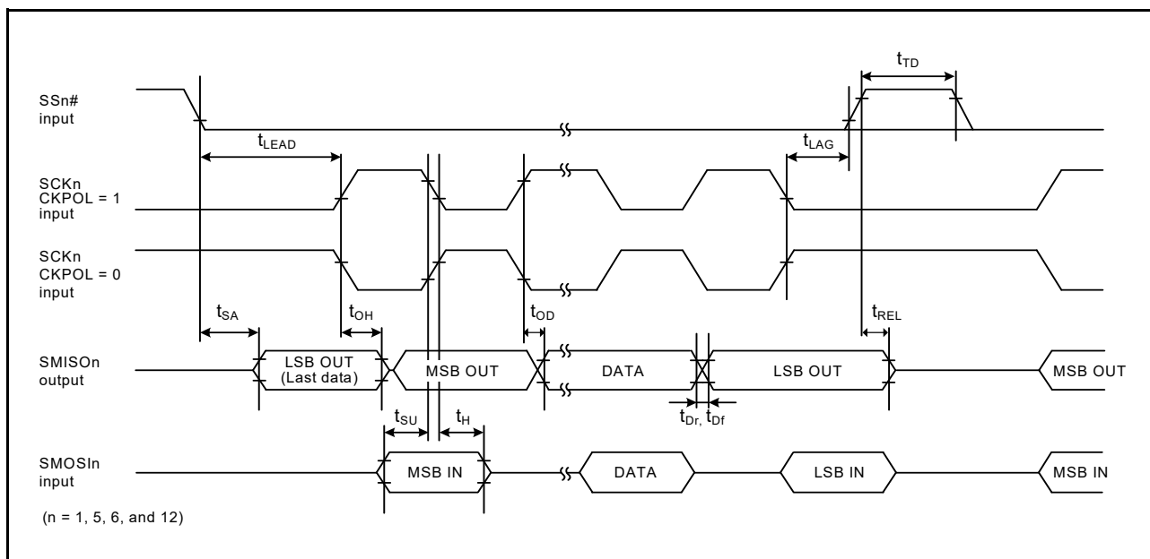
Figure 2.43 Simple SPI Timing (Slave, CKPH = 0)
