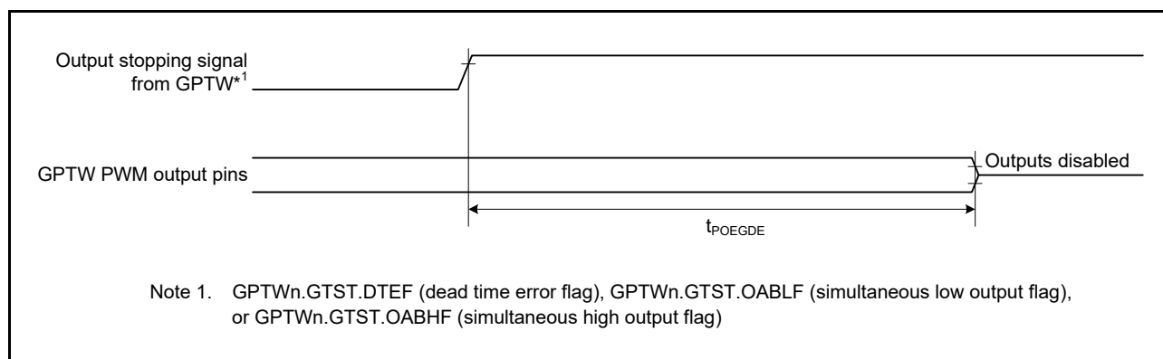
Figure 2.26 Output Disable Time for POEG in Response to Detection of the Output Stopping Signal from GPTW
