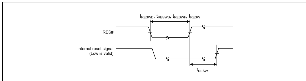
Figure 6.2 Reset Input Timing
