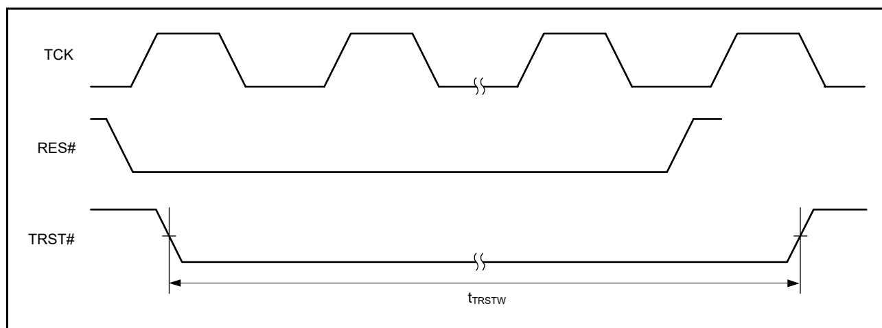
Figure 6.63 Boundary Scan TRST# Timing
