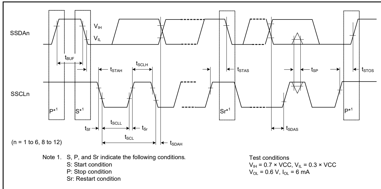
Figure 6.26 Simple IIC Bus Interface Input/Output Timing
