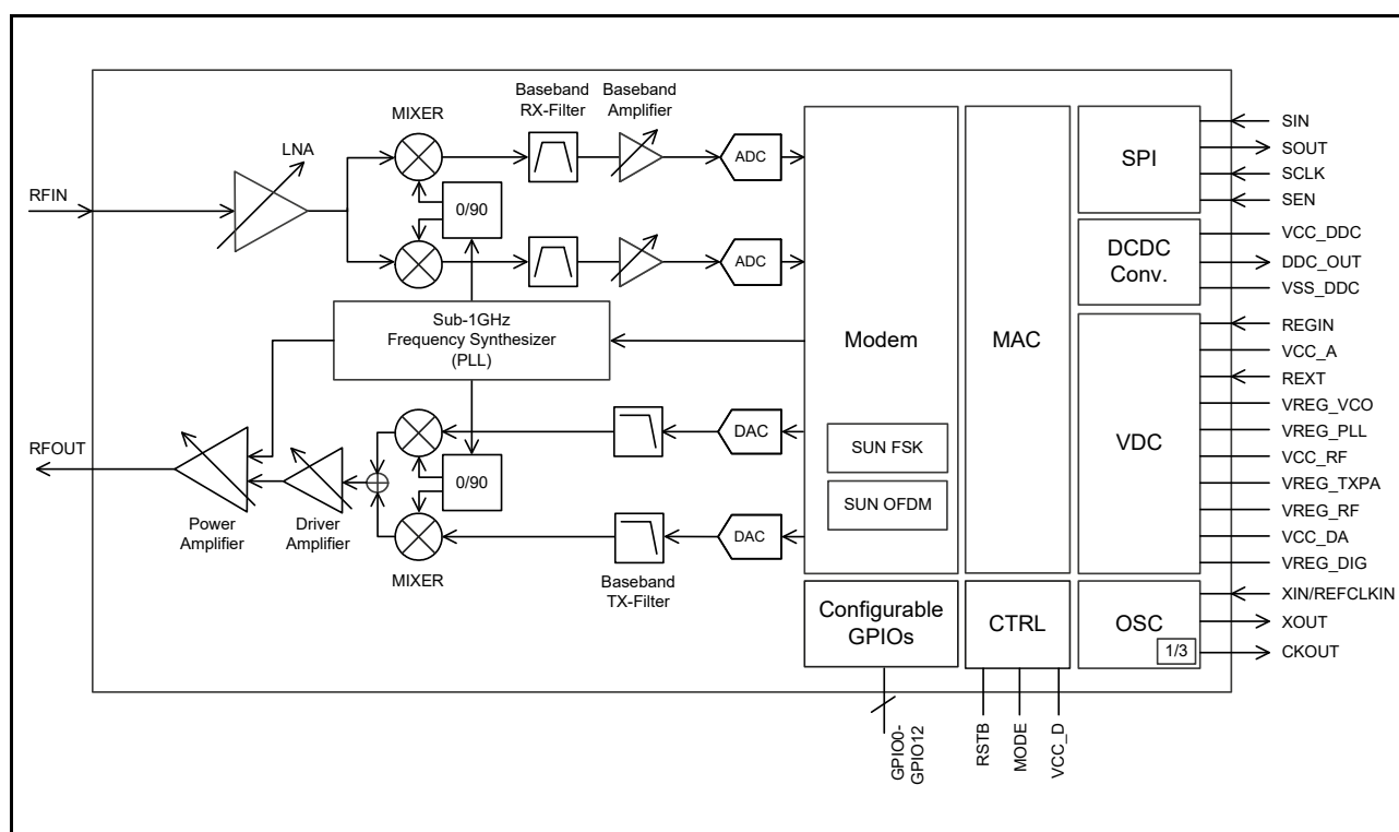
Figure 5.1 Block Diagram of RF Transceiver
