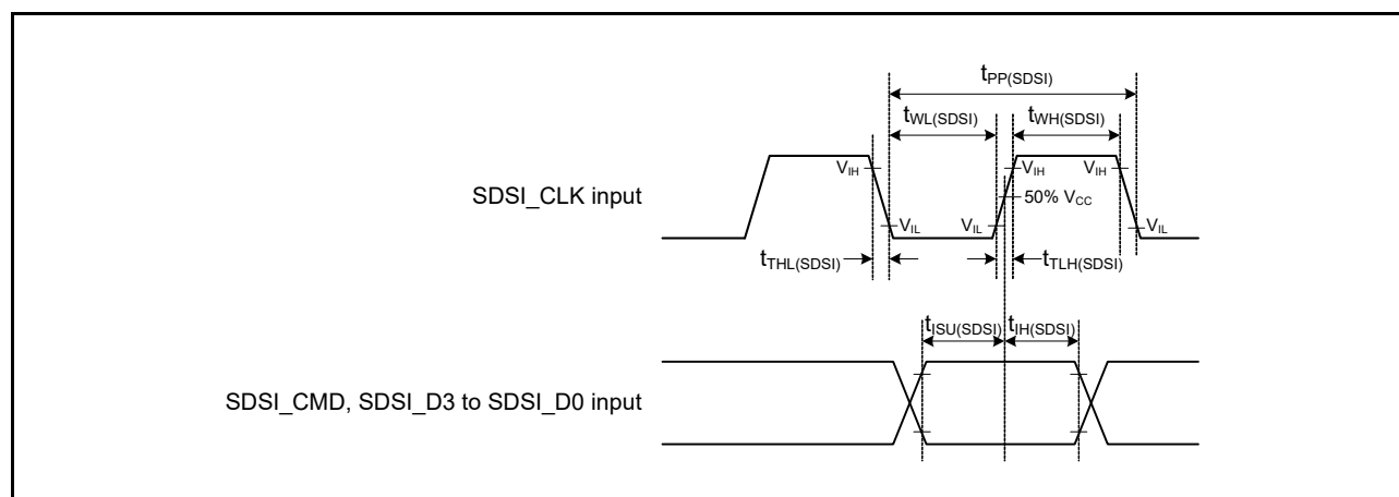
Figure 6.49 SD Slave Interface Input Signal Timing
