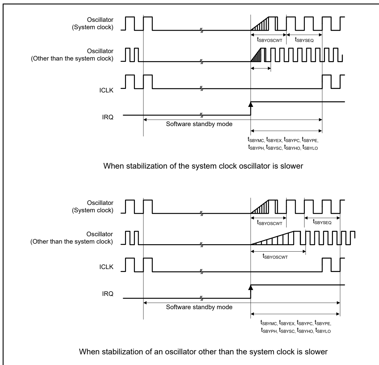
Figure 6.11 Software Standby Mode Recovery Timing
