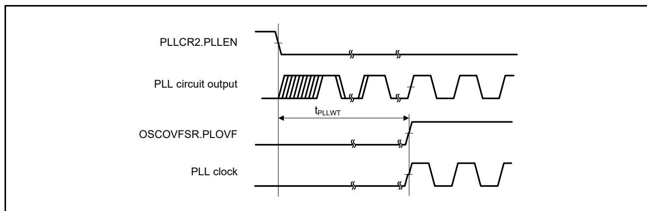
Figure 6.9 PLL Clock Oscillation Start Timing
