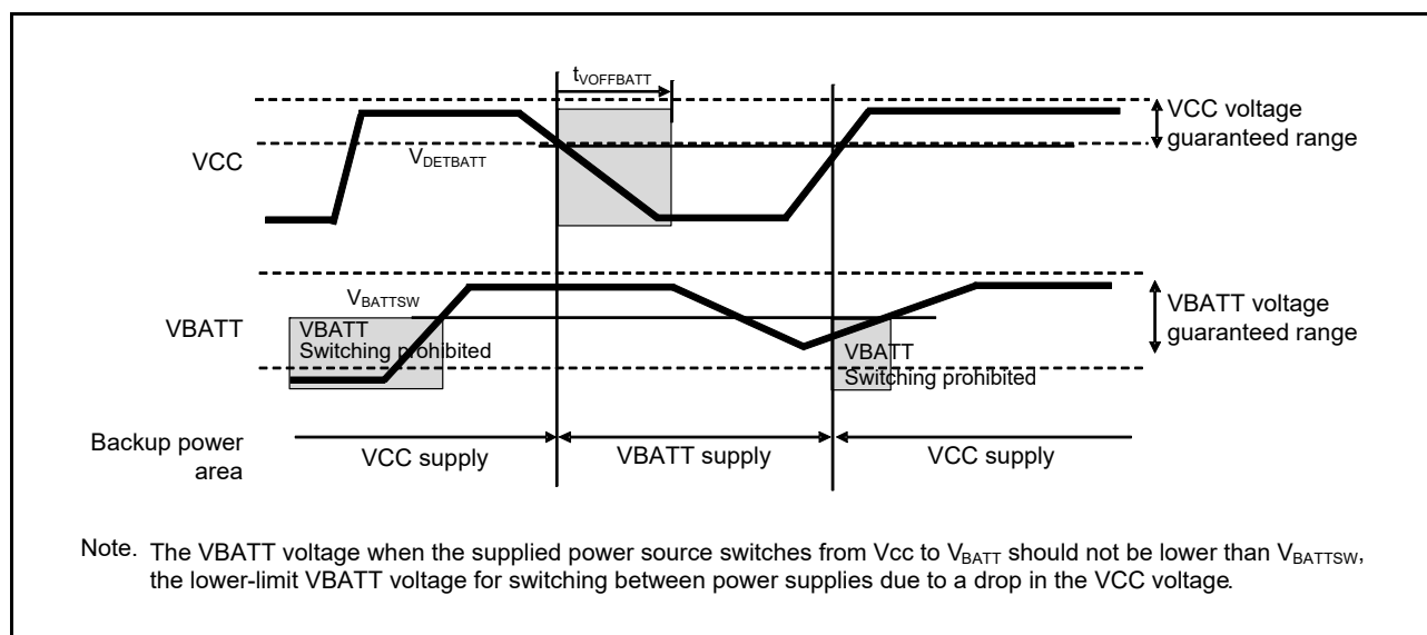
Figure 6.60 Battery Backup Function Characteristics
