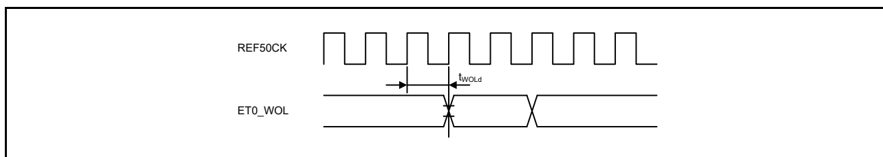
Figure 6.47 WOL Output Timing (RMII)
