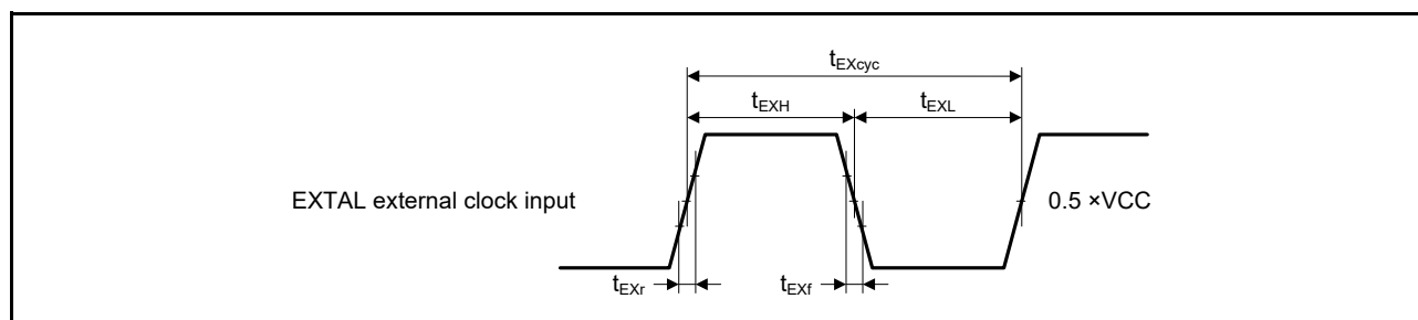
Figure 6.3 EXTAL External Clock Input Timing
