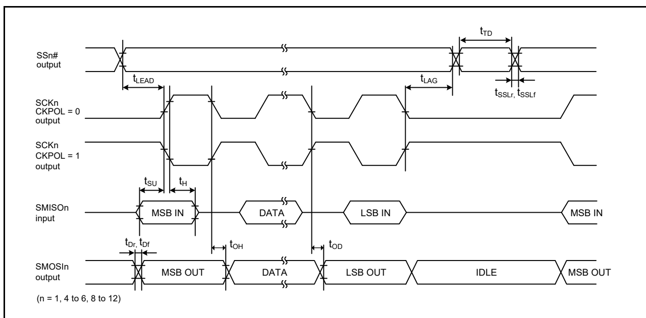
Figure 6.28 Simple SPI Timing (Master, CKPH = 1)
