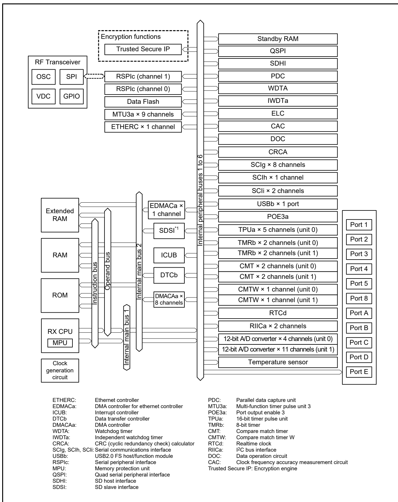
Figure 1.2 Block Diagram
