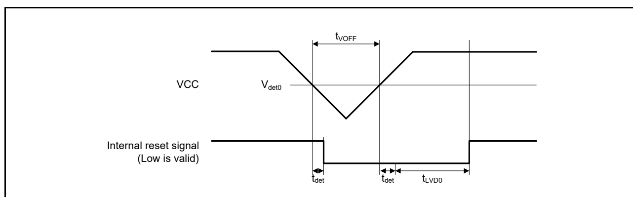
Figure 6.56 Voltage Detection Circuit Timing ( V_{det0} )
