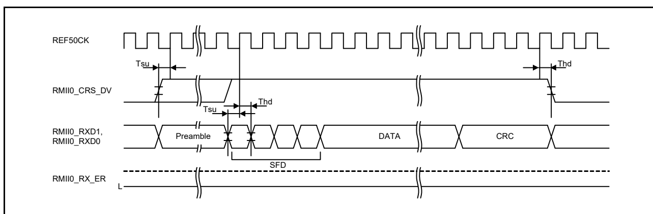
Figure 6.45 RMII Reception Timing (Normal Operation)
