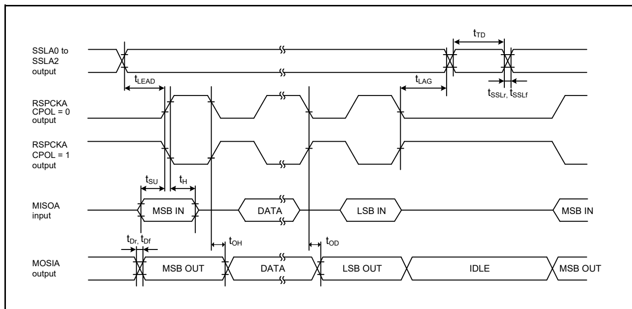
Figure 6.33 RSPI Timing (Master, CPHA = 0) (Bit Rate: PCLKA Division Ratio Set to a Value Other Than 1/2)
