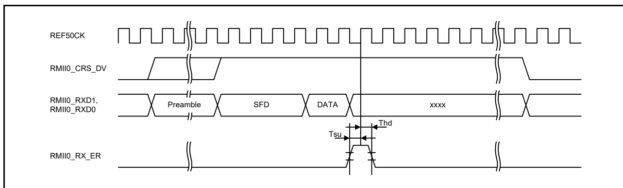
Figure 6.46 RMII Reception Timing (Error Occurrence)
