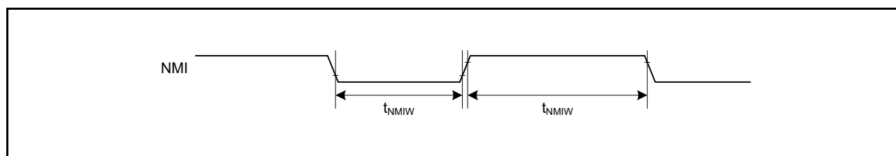
Figure 6.13 NMI Interrupt Input Timing
