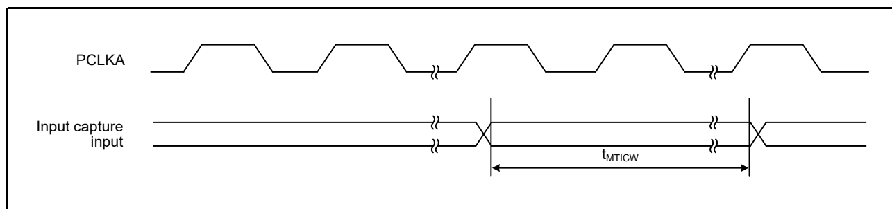
Figure 6.20 MTU3 Input Capture Input Timing
