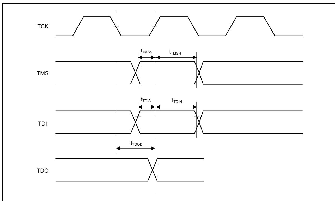
Figure 6.64 Boundary Scan Input/Output Timing
