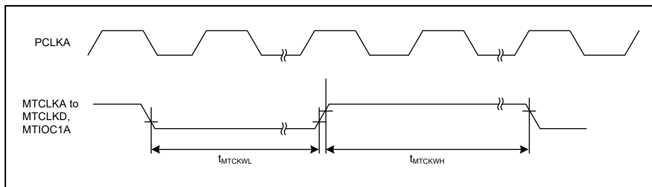
Figure 6.21 MTU3 Clock Input Timing
