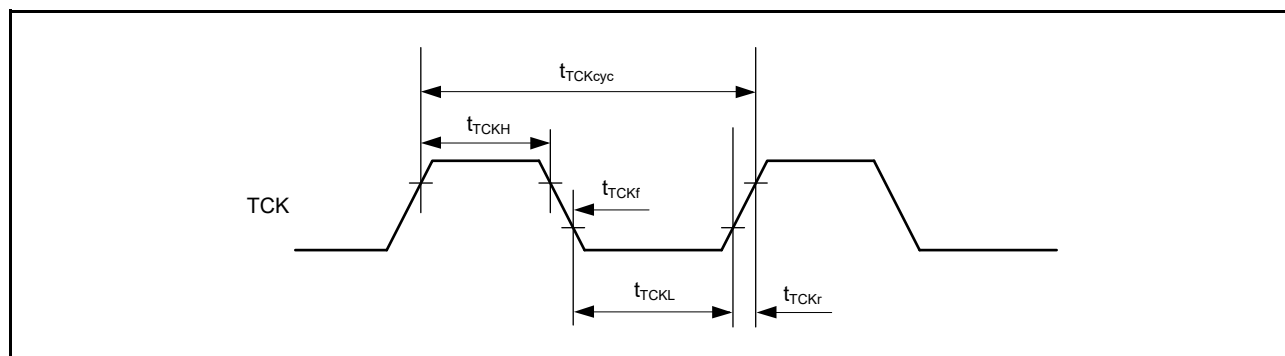
Figure 6.62 Boundary Scan TCK Timing
