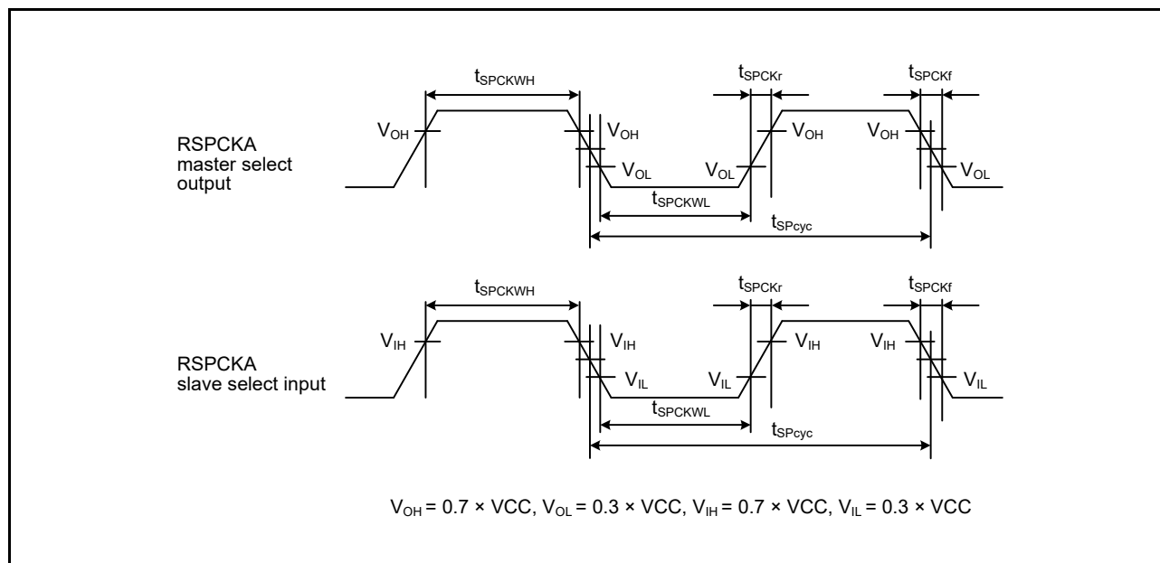
Figure 6.32 RSPI Clock Timing
