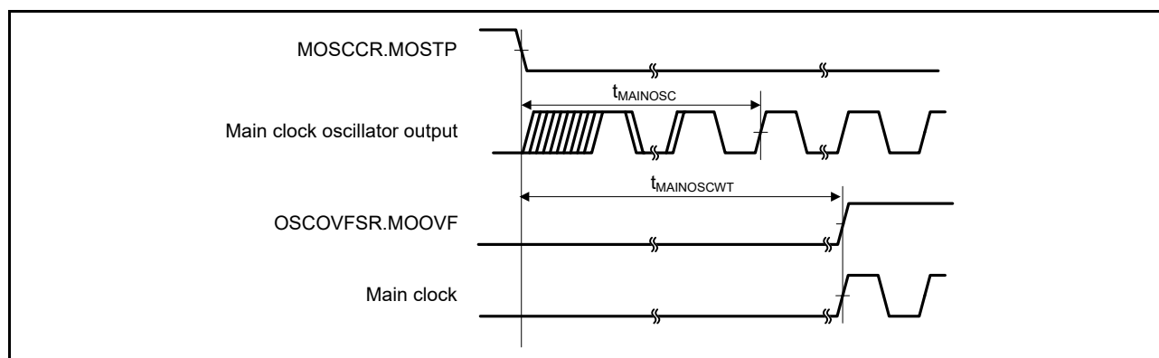
Figure 6.4 Main Clock Oscillation Start Timing
