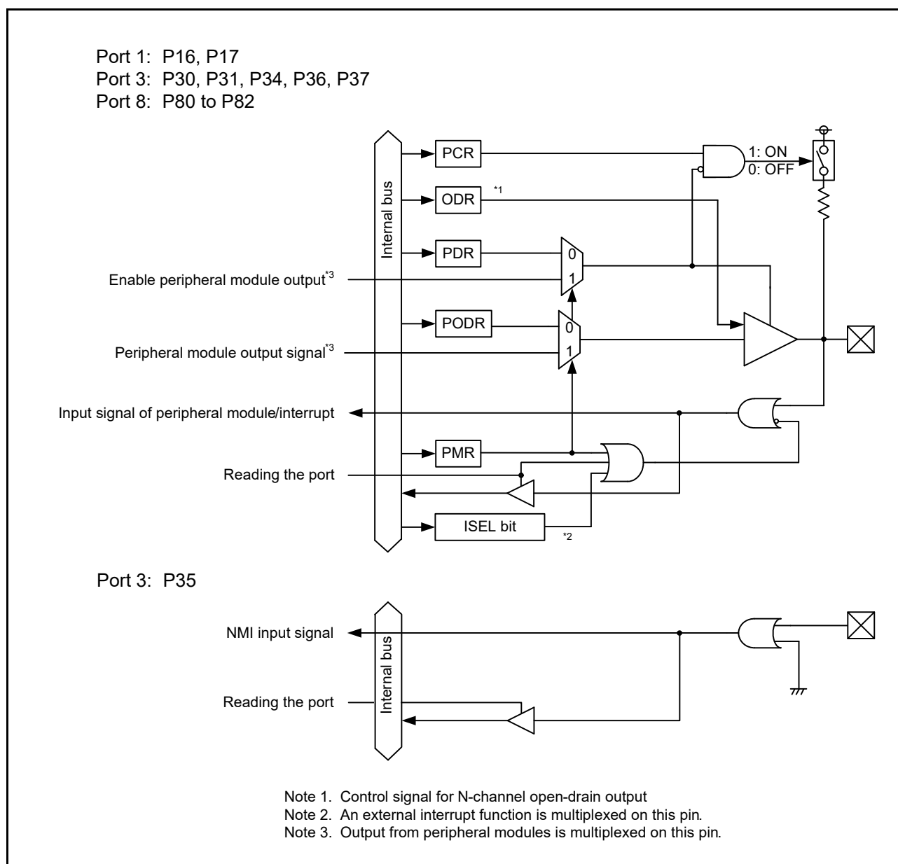
Figure 2.2 I/O Port Configuration (2)
