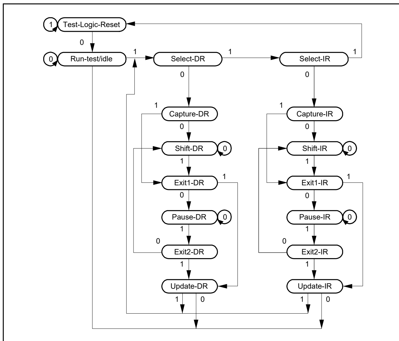
Figure 4.2 State Transition Diagram of TAP Controller
