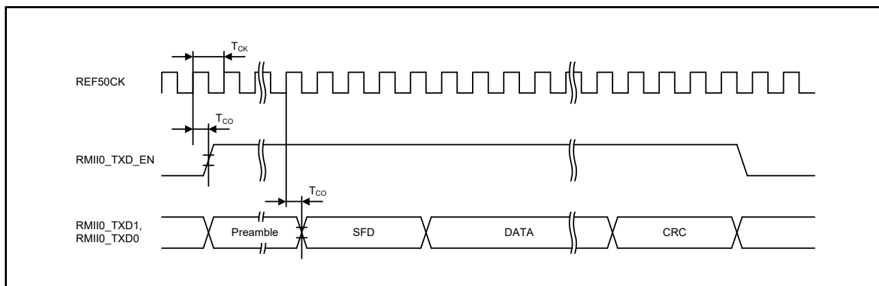
Figure 6.44 RMII Transmission Timing
