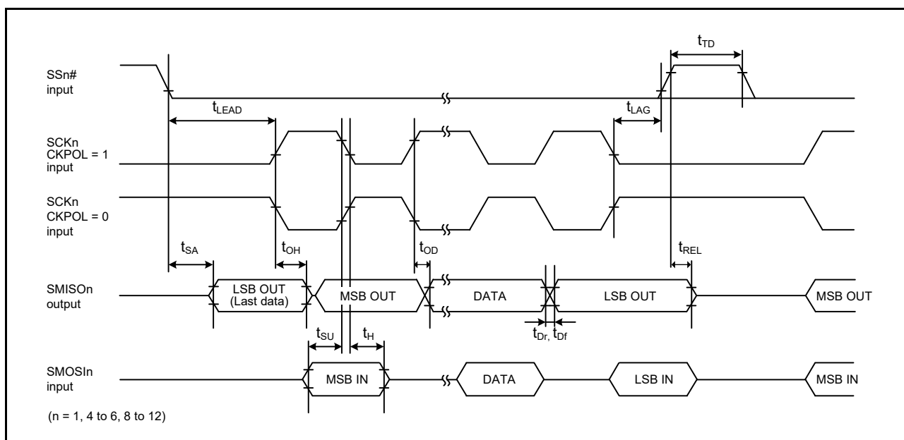
Figure 6.31 Simple SPI Timing (Slave, CKPH = 0)
