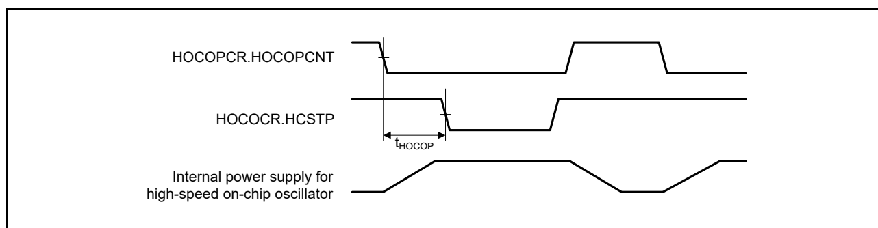
Figure 6.8 High-Speed On-Chip Oscillator Power Supply Control Timing
