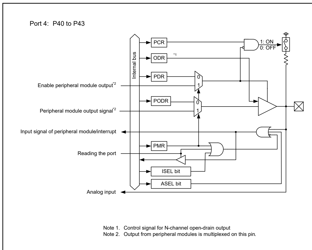
Figure 2.1 I/O Port Configuration (1)
