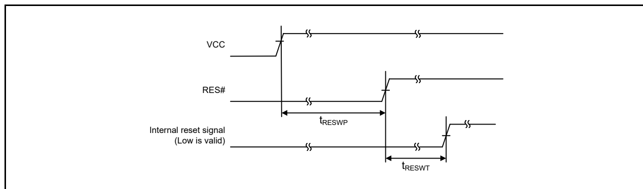
Figure 6.1 Reset Input Timing at Power-On
