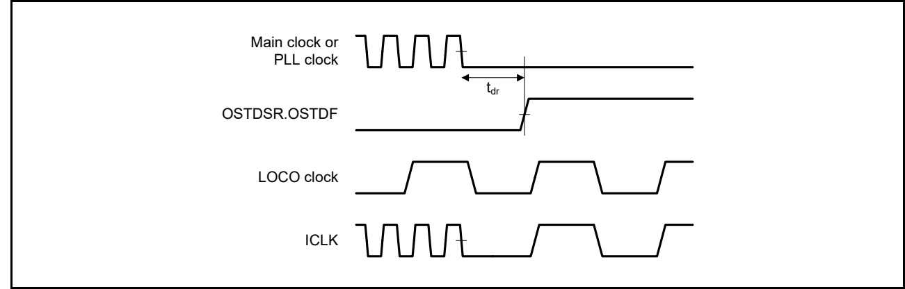
Figure 6.59 Oscillation Stop Detection Timing
