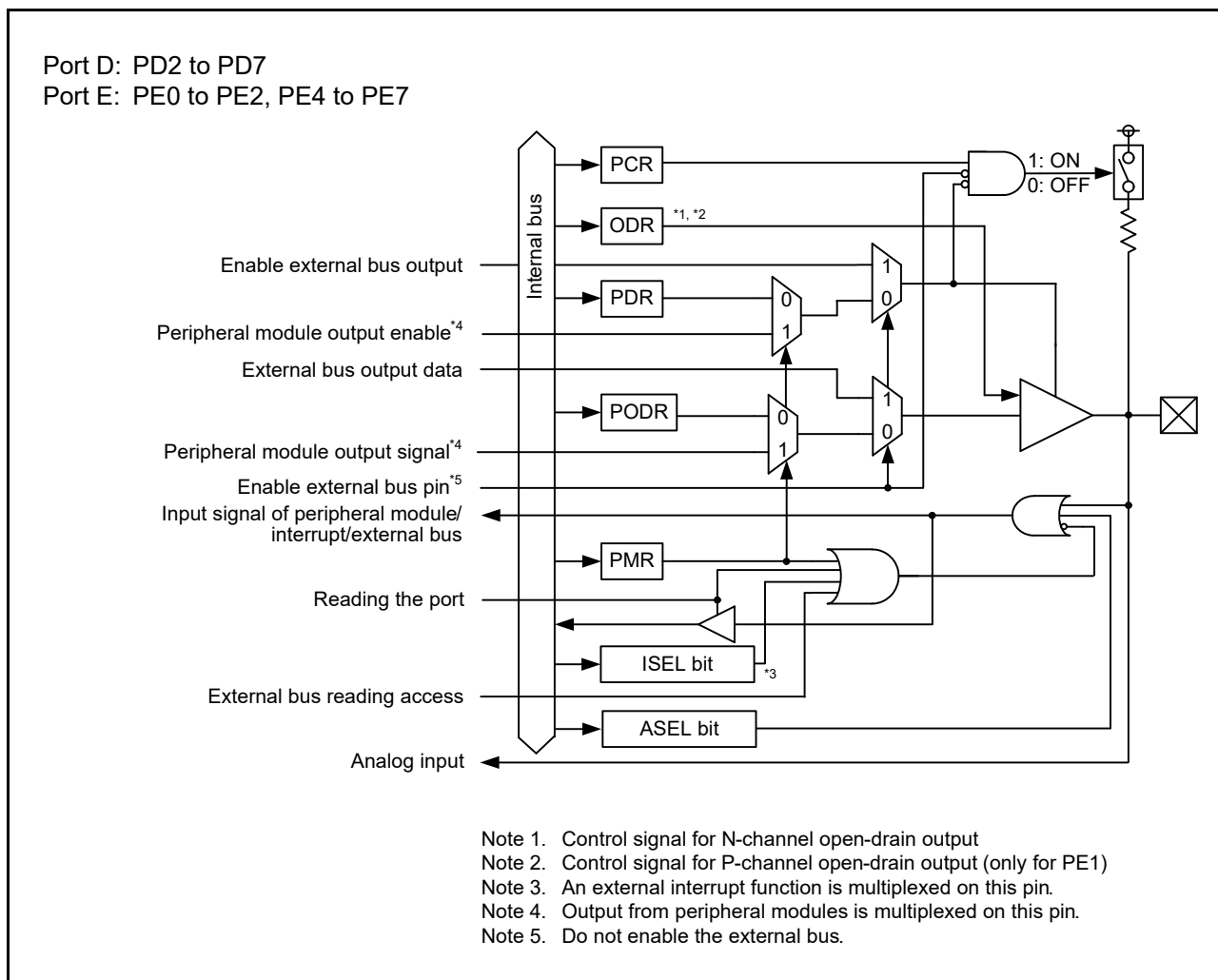
Figure 2.4 I/O Port Configuration (4)
