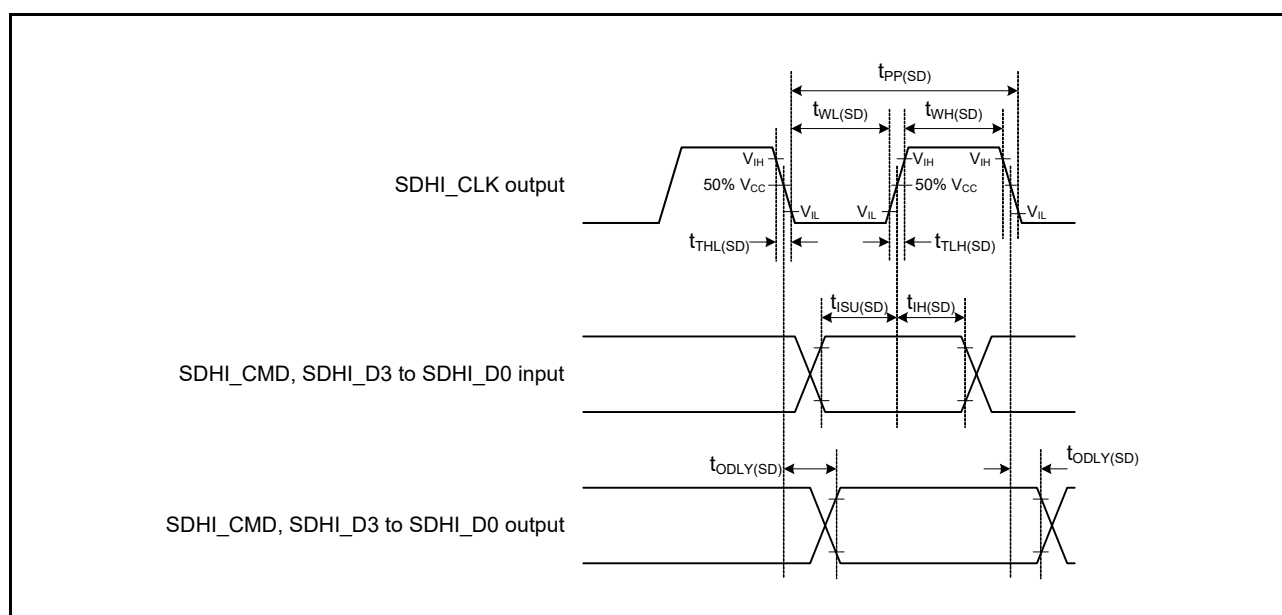
Figure 6.48 SD Host Interface Input/Output Signal Timing
