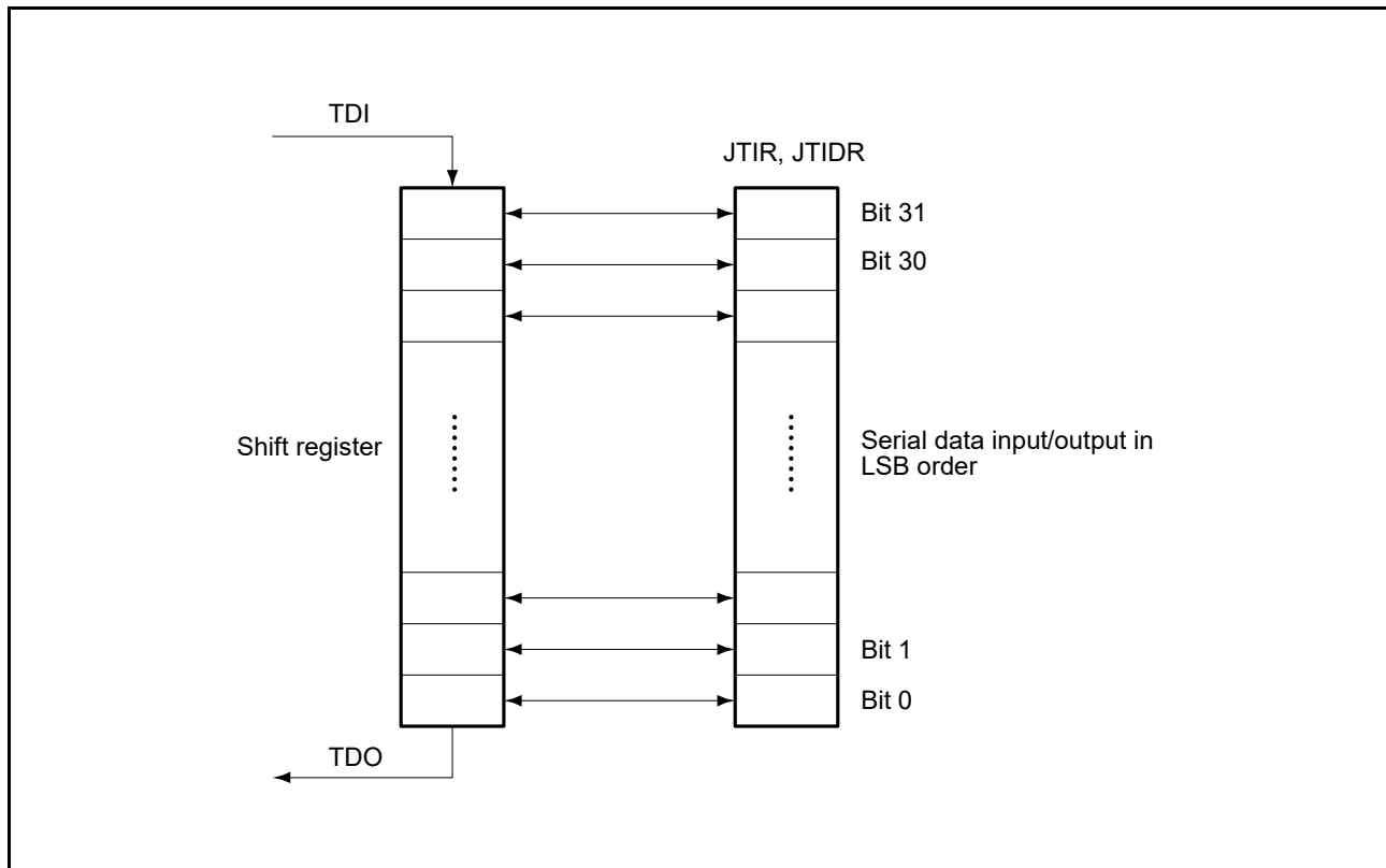
Figure 4.3 Serial Data Input/Output
