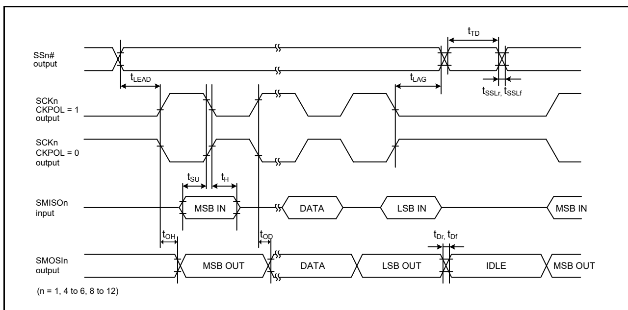
Figure 6.29 Simple SPI Timing (Master, CKPH = 0)
