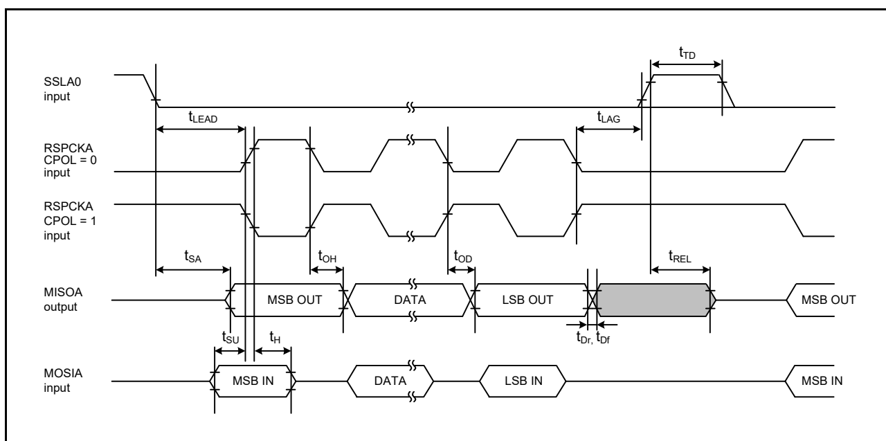
Figure 6.37 RSPI Timing (Slave, CPHA = 0)
