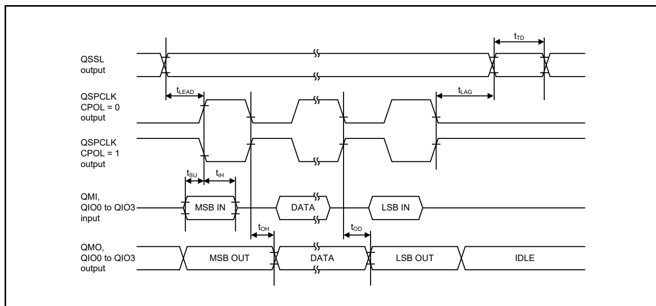
Figure 6.40 Transmit/Receive Timing (CPHA = 0)
