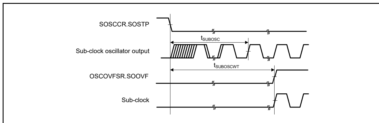
Figure 6.10 Sub-Clock Oscillation Start Timing
