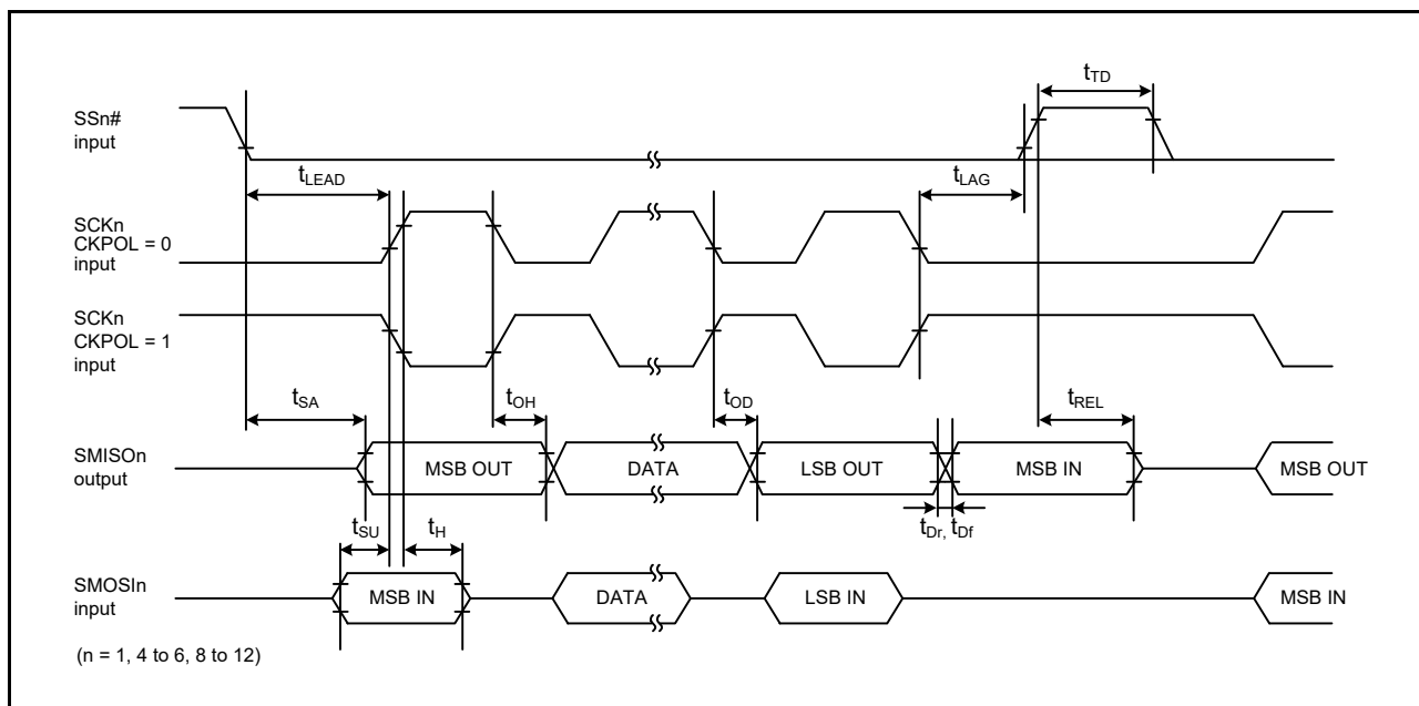
Figure 6.30 Simple SPI Timing (Slave, CKPH = 1)
