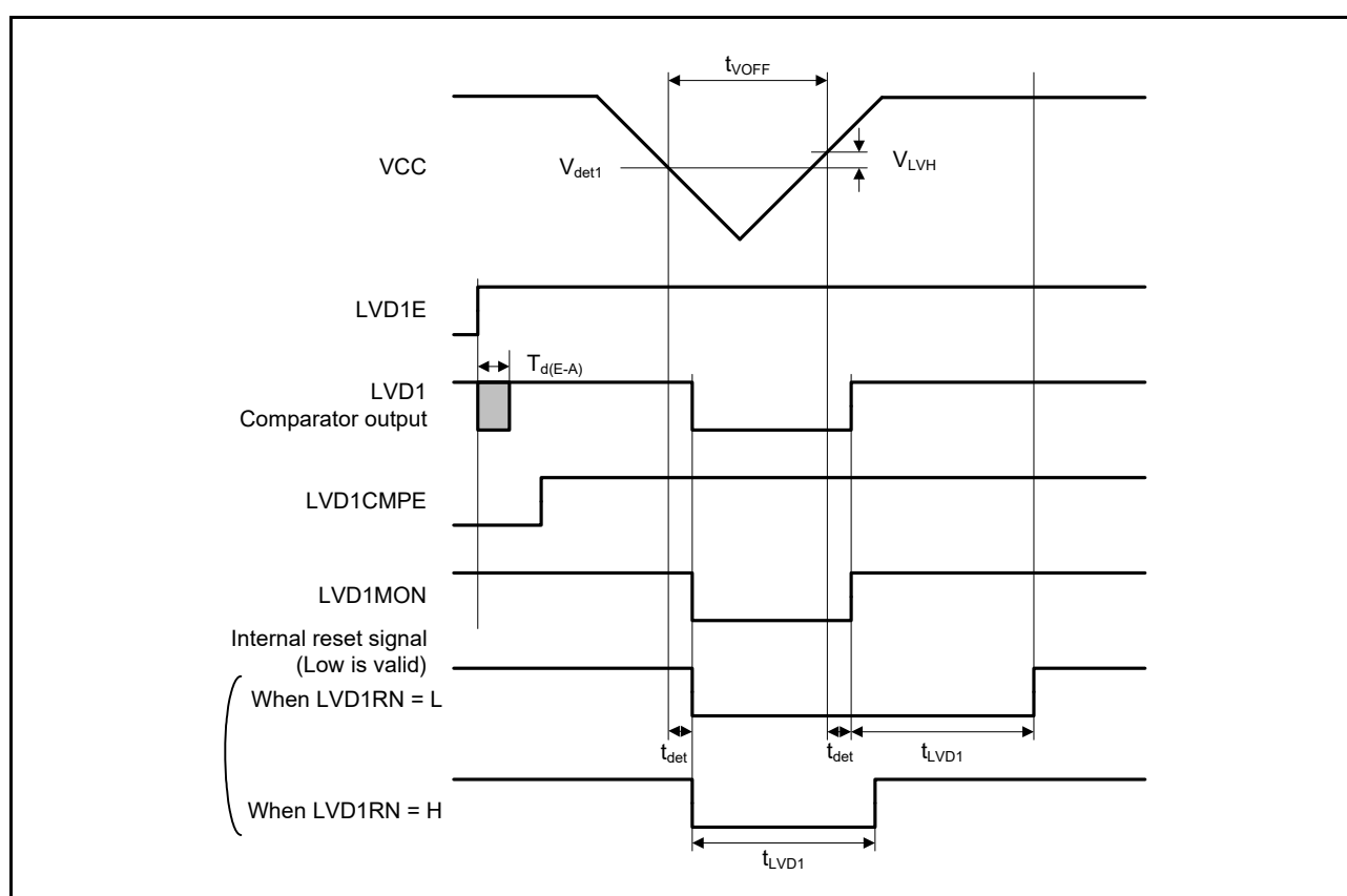
Figure 6.57 Voltage Detection Circuit Timing ( V_{det1} )
