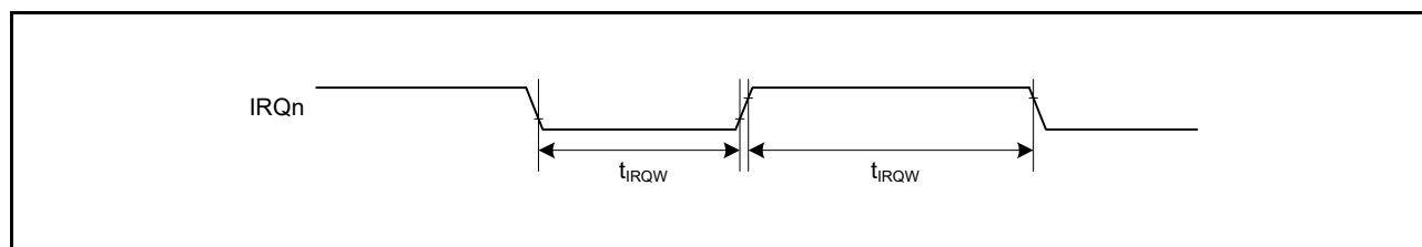
Figure 6.14 IRQ Interrupt Input Timing
