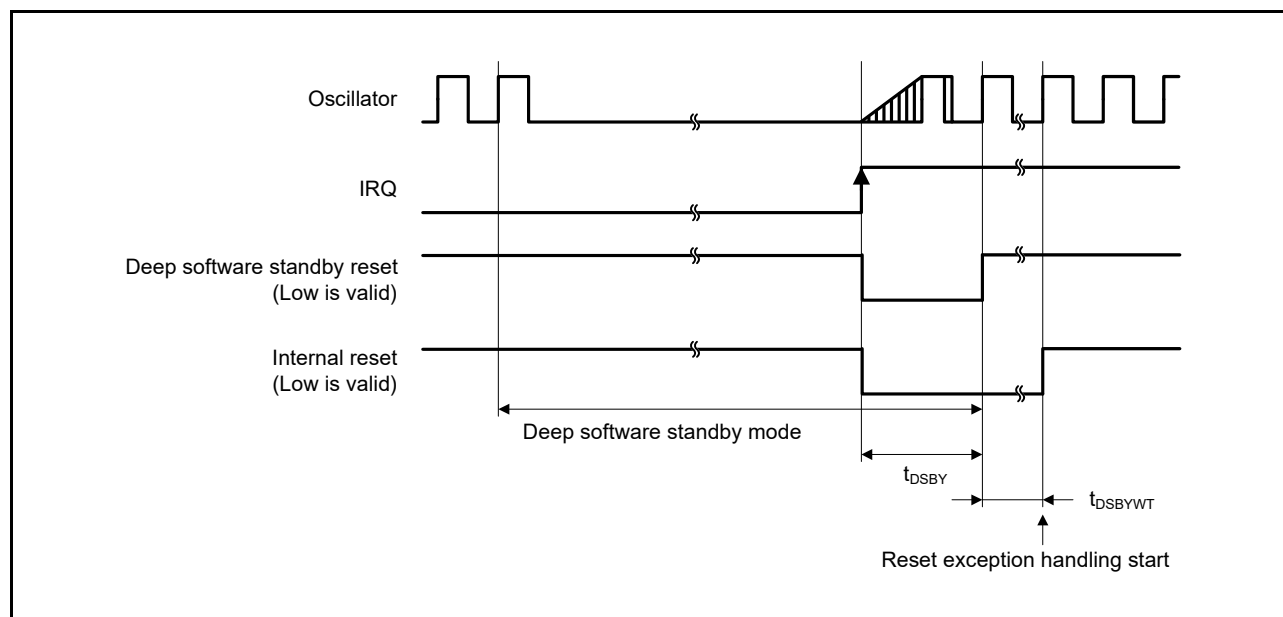
Figure 6.12 Deep Software Standby Mode Recovery Timing
