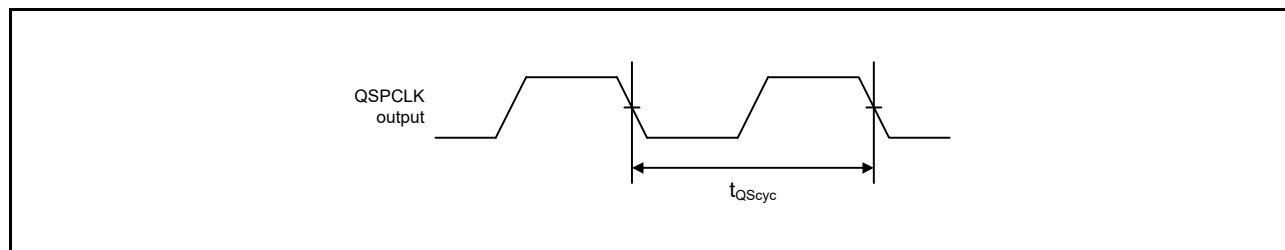
Figure 6.39 QSPI Clock Timing
