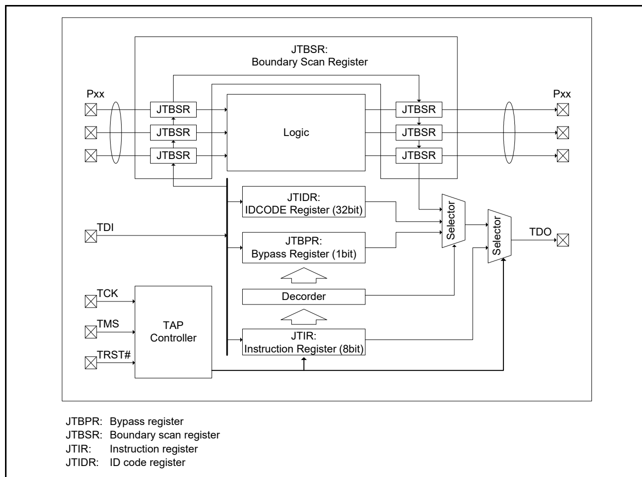
Figure 4.1 Block Diagram of JTAG
