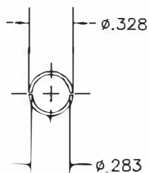
VIEW A
