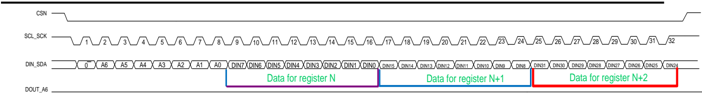
Figure 16.SPI Register Write Cycle - Burst (3-register burst example)
