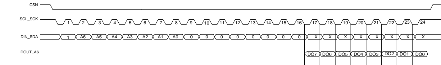
Figure 17. SPI Register Read Cycle - Single
