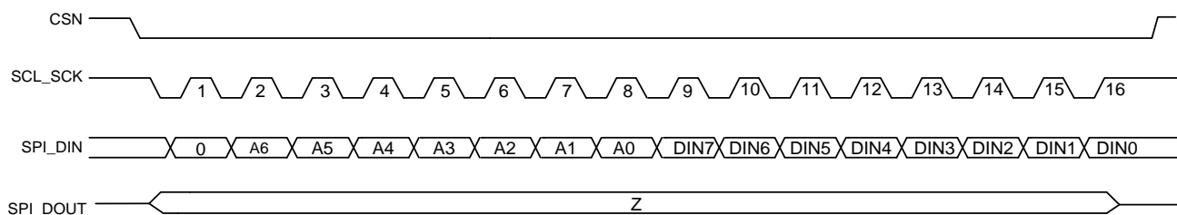
Figure 15. SPI Register Write Cycle - Single
