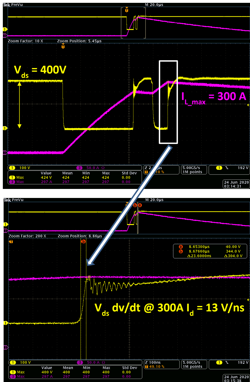
Figure 9 Double pulse test – High Side GaN Switching OFF waveforms
