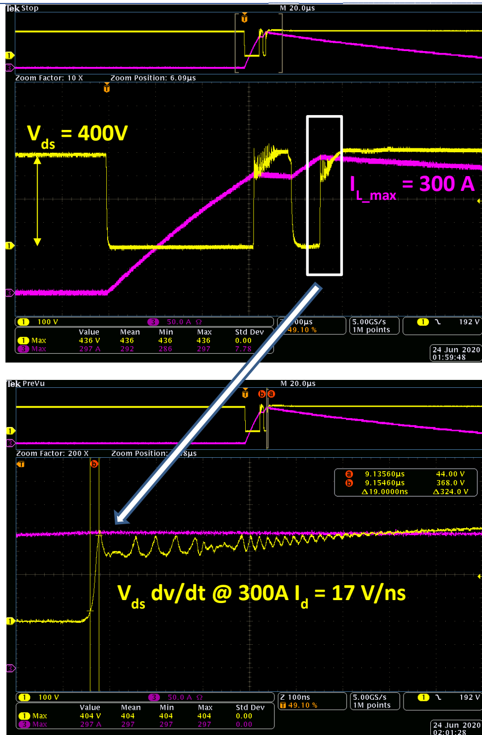
Figure 7 Double pulse test – Low Side GaN Switching OFF waveforms
