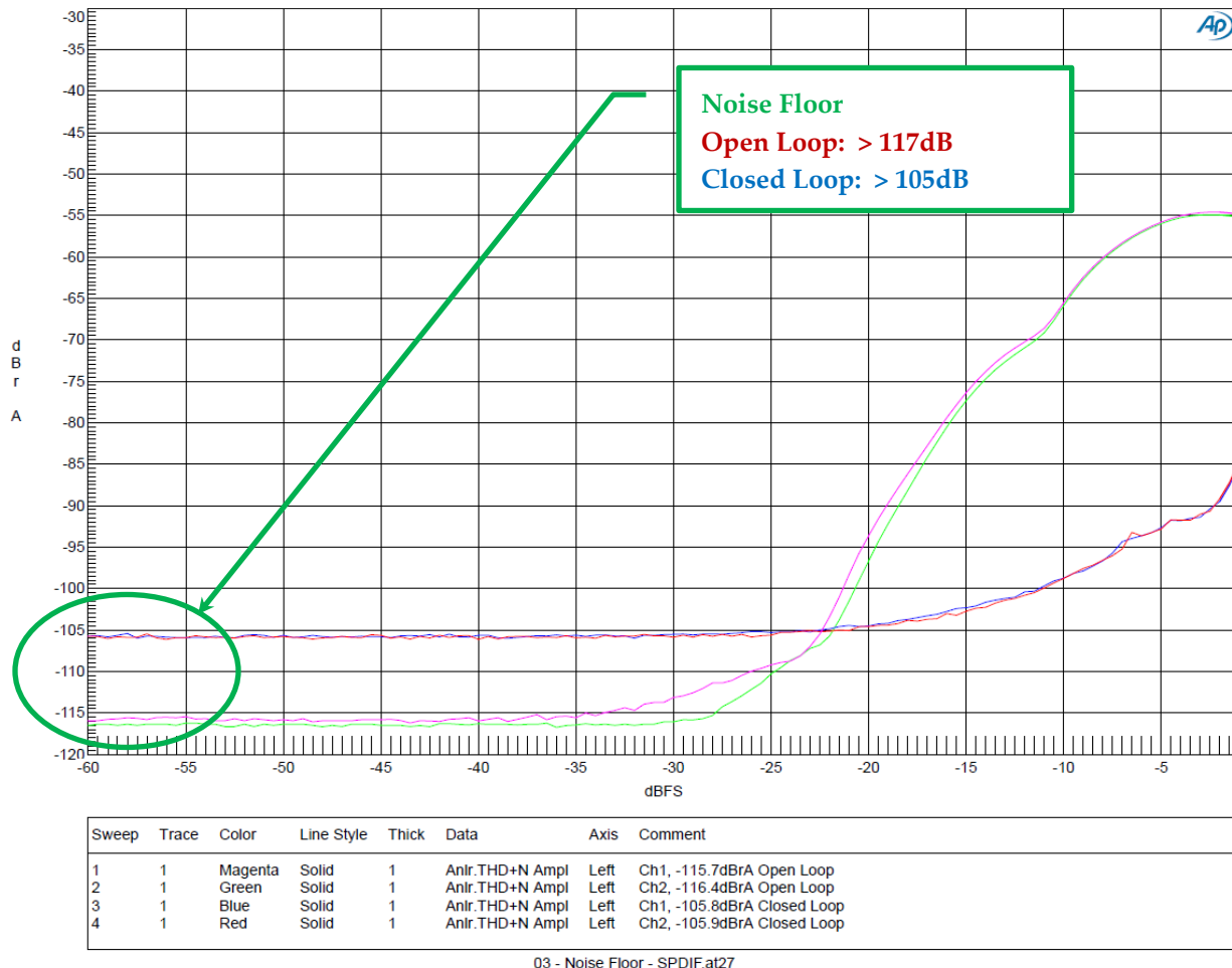
Figure 5. 3 Noise Floor
