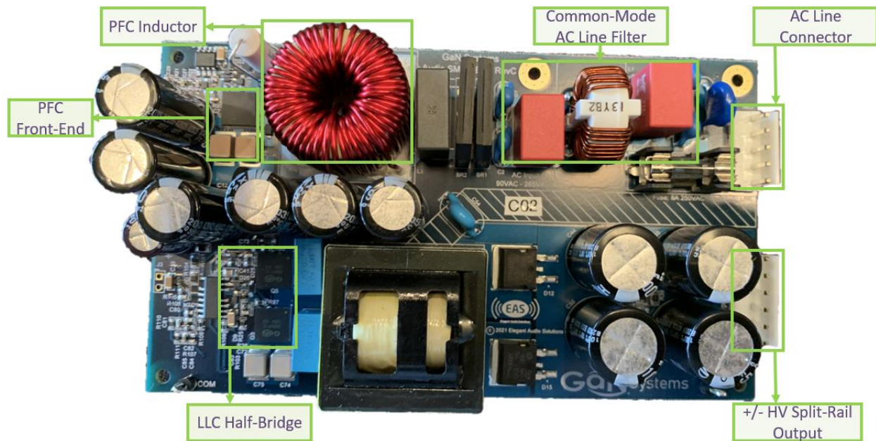
Figure 2. 2 GaN-based LLC SMPS w/PFC
