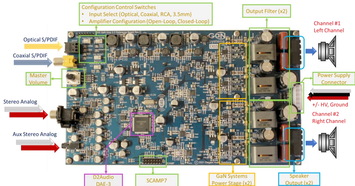
Figure 2. 3 Stereo Class-D GaN E-HEMT Audio Amplifier Reference
