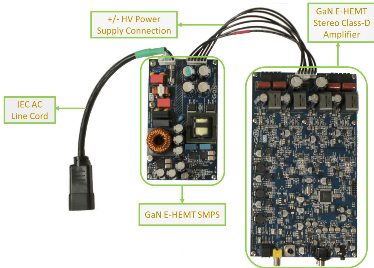
Figure 2. 1 Complete GaN Systems Audio Amplifier Platform
