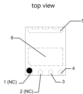
Package Outline
