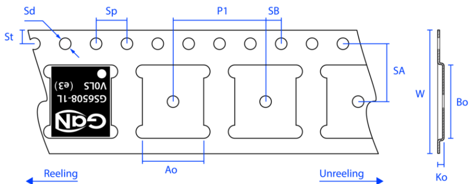
Dimensions (mm)
