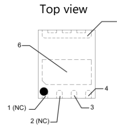
Package Outline
