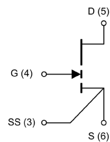
Circuit Symbol
