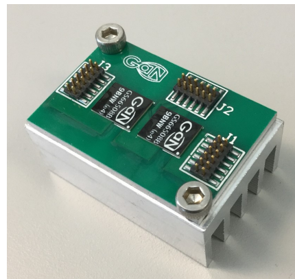
Figure 1 IMS 2 EVB board and IMS 2 half bridge power module with heatsink
