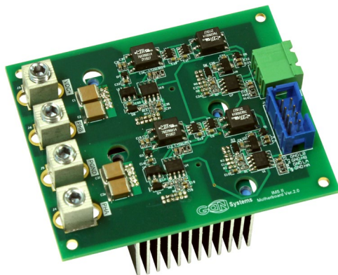
Figure 1 IMS 2 EVB board and IMS 2 half bridge power module with heatsink
