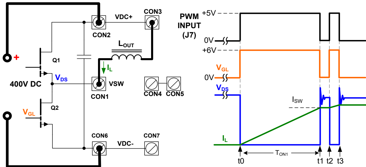
Figure 15 Double pulse test setup
