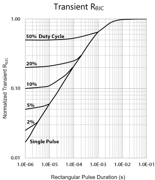
Figure 15: Transient Thermal Impedance (1.00 = Nominal DC thermal impedance)
