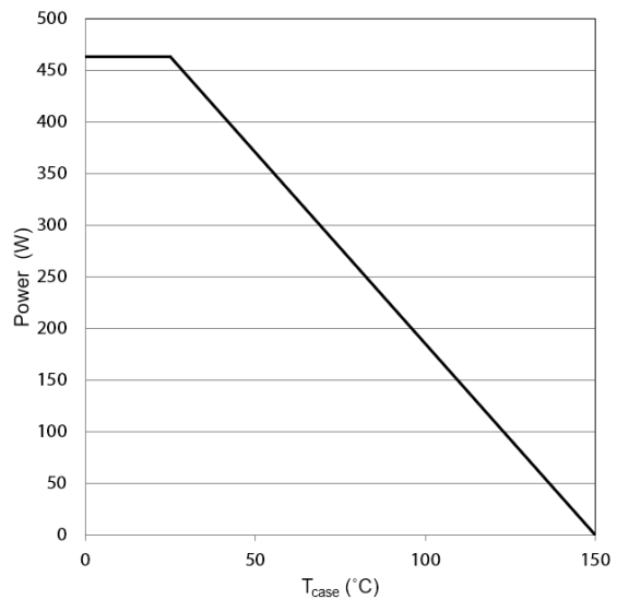
Figure 14: Derating vs. Case Temperature
