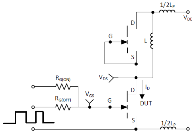
Figure 17: Switching Loss Test Circuit
