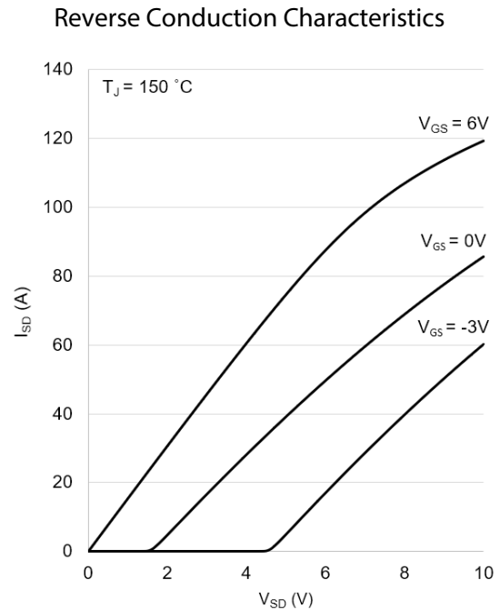
Figure 10: Typical I_{SD} vs. V_{SD} , T_J = 150\text{ }^{\circ}\text{C}
