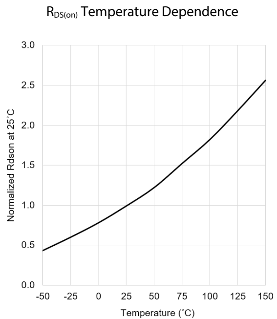
Figure 12: Normalized R_{DS(on)} as a function of T_J
