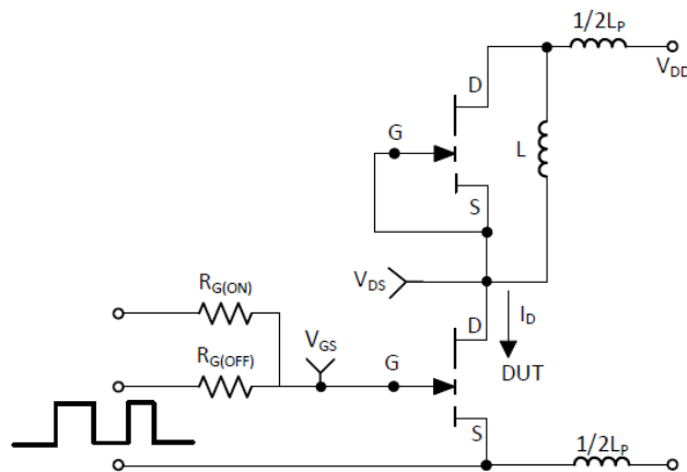
Figure 17: Switching Loss Test Circuit
