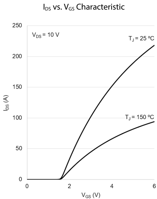
Figure 11: Typical I_{DS} vs. V_{GS}
