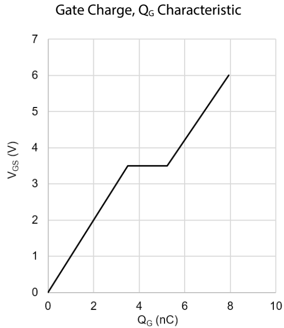
Figure 6: Typical V_{GS} vs. Q_G @ V_{DS} = 50V
