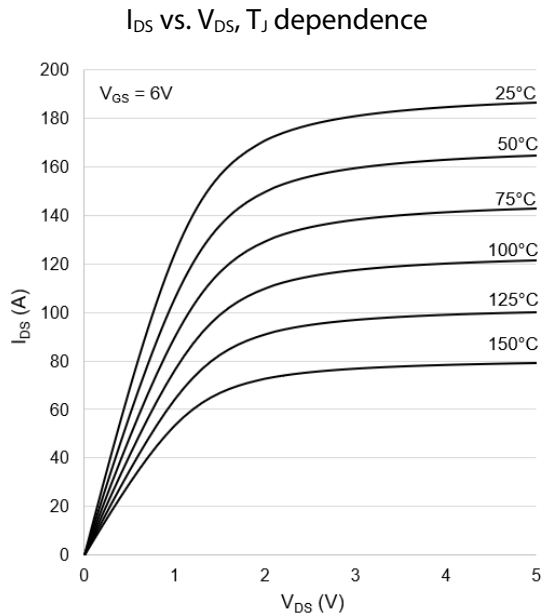
Figure 5: Typical I_{DS} vs. V_{DS} @ V_{GS} = 6V
