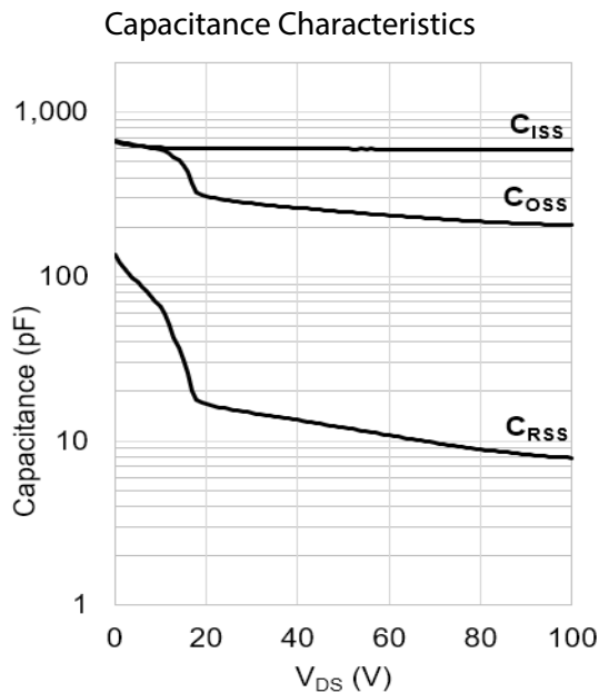
Figure 7: Typical C_{ISS} , C_{OSS} , C_{RSS} vs. V_{DS}
