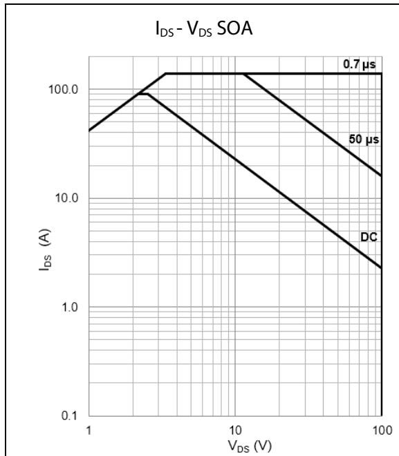
Figure 13: Safe Operating Area @ T_{case} = 25^\circ\text{C}
